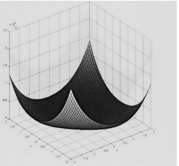
Figure 56: Perm #2 function
