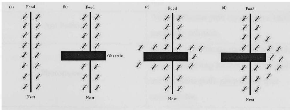
Figure 8: Pheromone explanation
