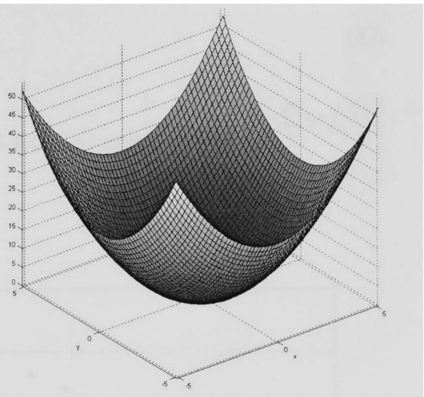
Figure 58: Sphere function
