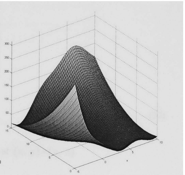
Figure 26: Branin function
