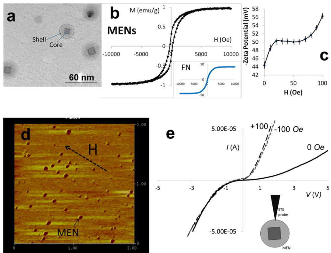
Figure 1. MENs' physical properties. (a) Transmission Electron Microscopy (TEM) image showing the coreshell nanostructure of MENs (spinel \text{CoFe}_2\text{O}_4 core and perovskite \text{BaTiO}_3 shell). (b) M-H hysteresis loop of MENs. The insert shows a loop for FNs. (c) Magnetic field dependence of Zeta Potential for 0.5 mg of MENs in a 1-ml PBS buffer solution with a pH of 7.3. (d) Magnetic force microscopy (MFM) image showing the dipole nature of 30-nm MENs. (e) Scanning Tunneling Spectroscopy (STS) I-V curve measured from a point contact between the tungsten nanoprobe of a STM setup and a MEN at three different field values, -100 , 0 , and 100 Oe, respectively, with a magnetic field applied along the central axis.
