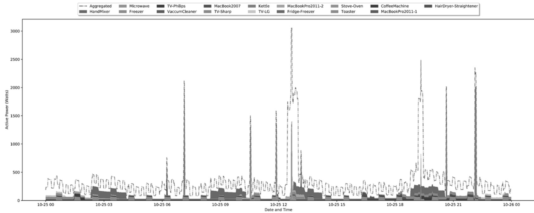
Figure 10: Example of Residential Watts, per device, throughout the day
