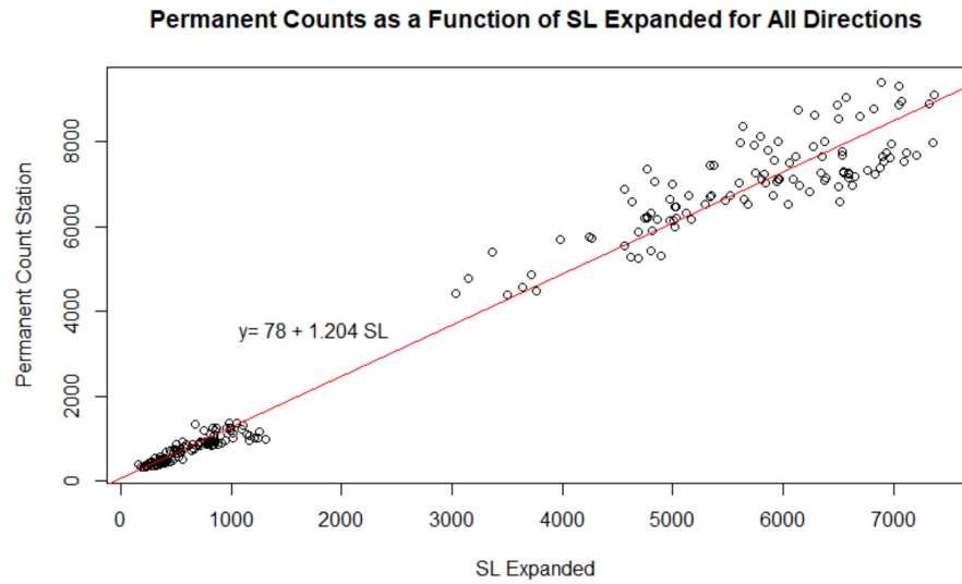
Figure 5-16 PCS Counts vs. SL Expanded fitted regression model for All Directions using hourly volumes (Scenario 2)
