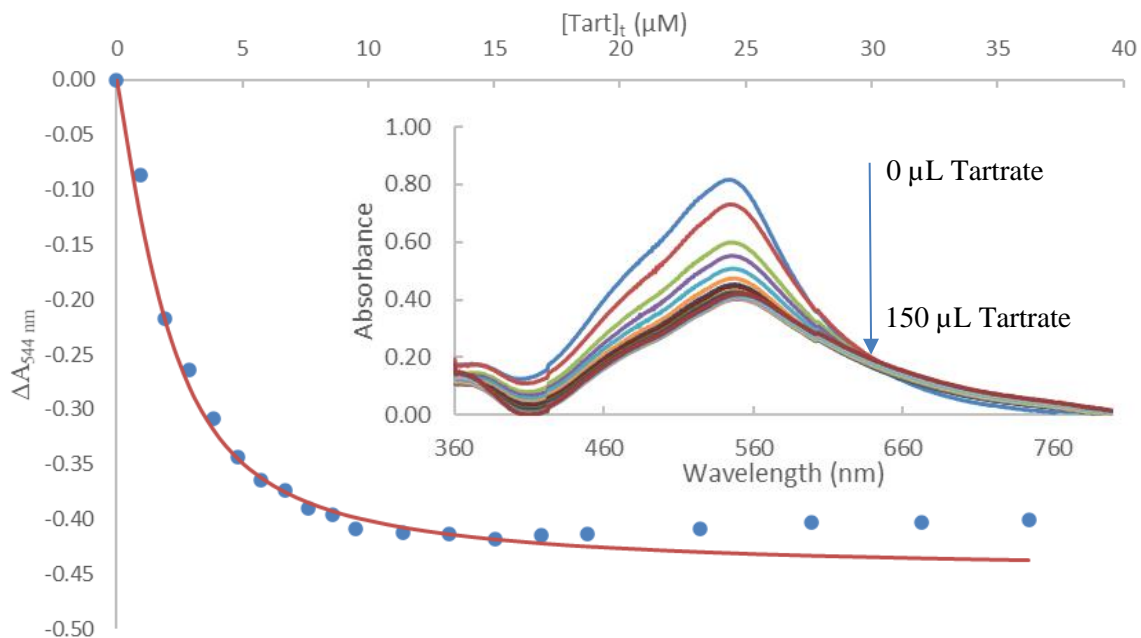
Figure 2.11: Binding curve for the titration of a solution of 2.00 \times 10^{-6} M of 1S with solution of 5.80 \times 10^{-4} M of pH 2.8 tartarate buffer in 2.00 \times 10^{-6} M of 1S in water/ethanol (50/50 v/v). K_{11} = 1.00 \times 10^6 \text{ M}^{-1} . Cutaway: UV-Visible absorption spectrum for the titration of a solution of 2.00 \times 10^{-6} M of 1S with a solution of 5.80 \times 10^{-4} M of pH 2.8 tartarate buffer in 2.00 \times 10^{-6} M of 1S in water/ethanol (50/50 v/v).
