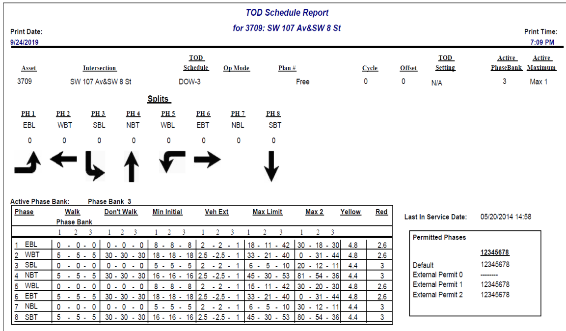
Figure 3-3: An Example of a Signal Timing Plan
