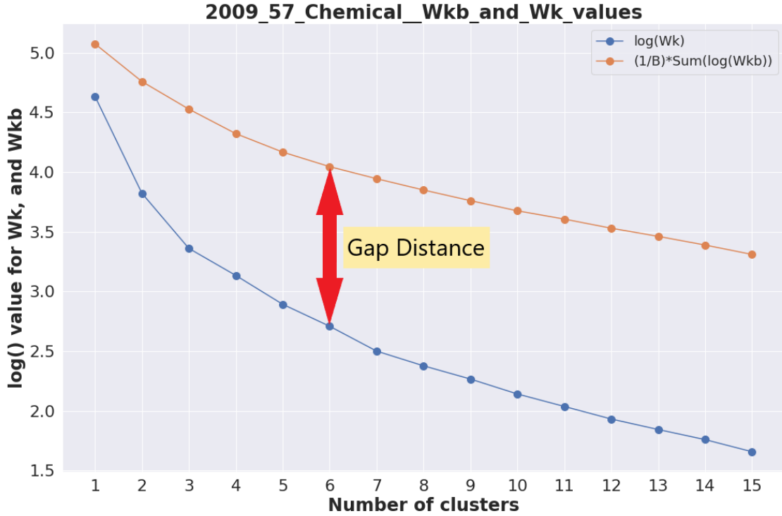
Figure 4.7: The gap distance is obtained from the difference between \log W_k (blue line) and (1/B) \sum_b \log (W_{kb}^*) (orange line). The values obtained will be used to graph distance curve as seen in figure 4.8
