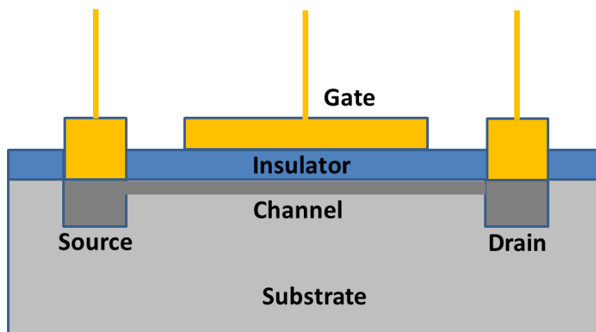
Figure 7: A typical top gated Si thin film transistor
