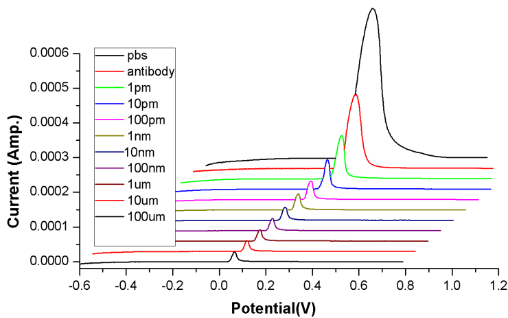
Figure 18: Different concentration of cortisol dispersed on the immunosensor and their oxidation response current.
