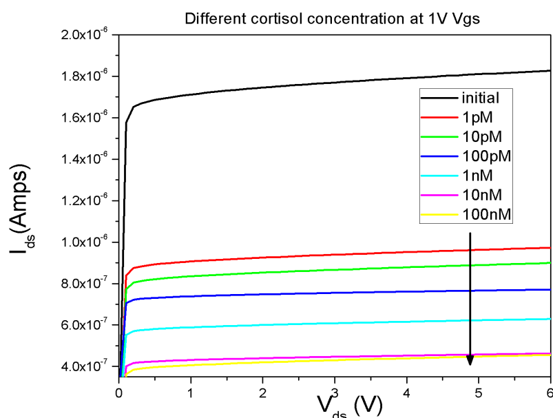
Figure 36: Different cortisol concentration at a lower gate voltage(1V). The reduction in drain current with increasing cortisol can be hypothesized due to cortisol molecules occupying empty sites in the MIP matrix and reducing electron transport in the polymer matrix. The reduced gate current, causes a reduction in the accumulated charges at the actual gate. Thus, causing a decrease in source drain current due to the reduced gate voltage.
