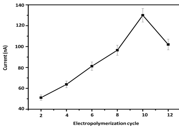
Figure 25: Effect of the different cycles of the electro polymerization of MIP constant concentration of cortisol (10 mM) and different pyrrole concentrations in the range of 0.2 M to 1.2 M (Figure 24). The polymerization and elution of cortisol to form MIP electrodes were followed as mentioned in the previous section. The
