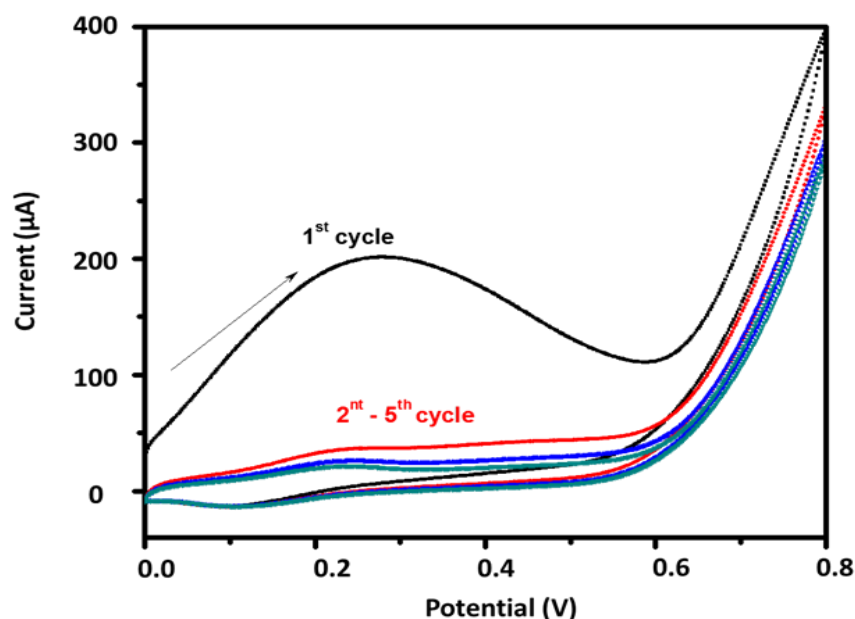
Figure 20: Recorded voltammograms during the elution of cortisol from the PPy matrix at 0.1 M PBS; scan rate of 50 mV/s.
