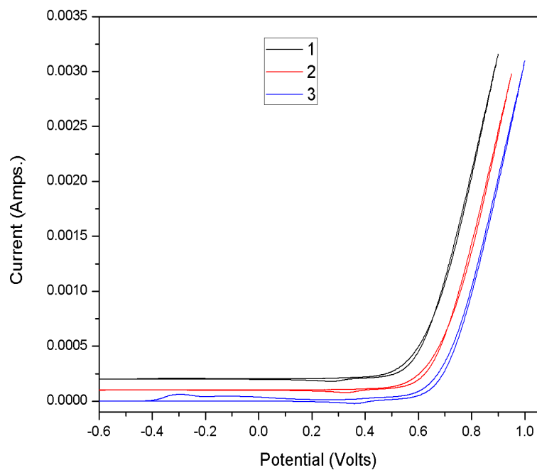
Figure 14: CV of copper nanoparticles being overoxidized for three cycles
