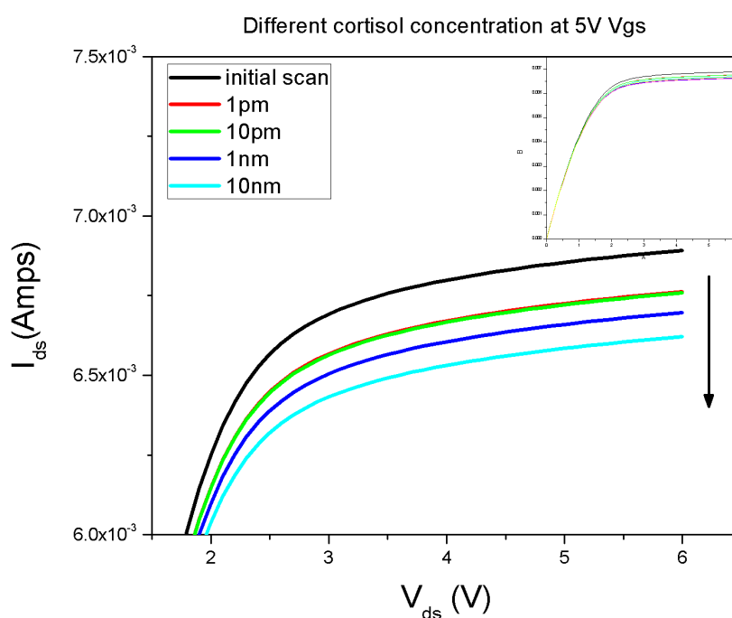
Figure 35: Output characteristics of the EGFET after adding different cortisol concentrations at a constant gate voltage of 5V
