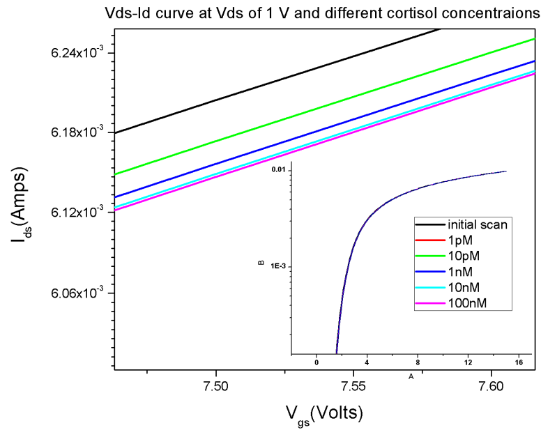
Figure 38: V_{gs} - I_d curve of the EGFET-MIP device at different cortisol concentrations. The drain voltage was kept as 1V
