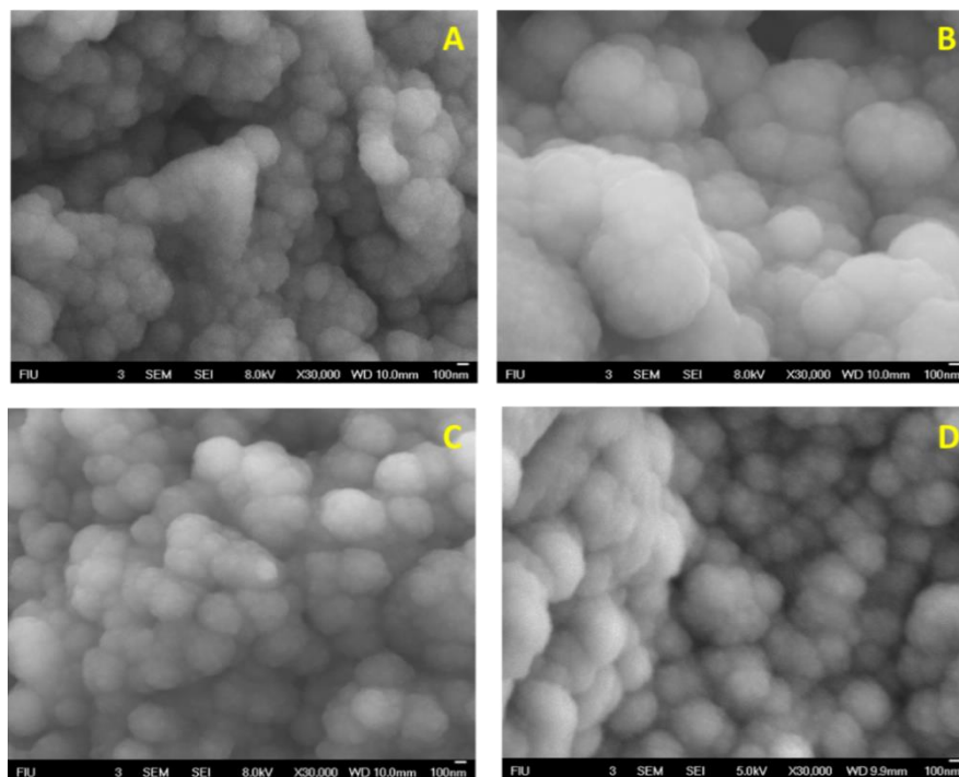
Figure 22: SEM images of (A) PPy-SPCE, (B) Cortisol-PPy-SPCE, (C) MIP-PPy-SPCE, and (D) NIP-PPy-SPCE
