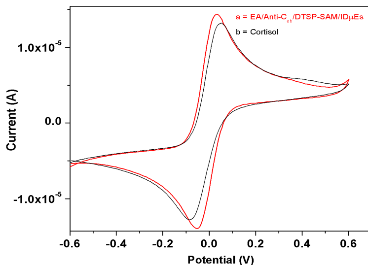
Figure 10: Electrochemical response of EA/Anti-C ab /DTSP-SAM/IDEs immunoelectrode after addition of standard cortisol solution
