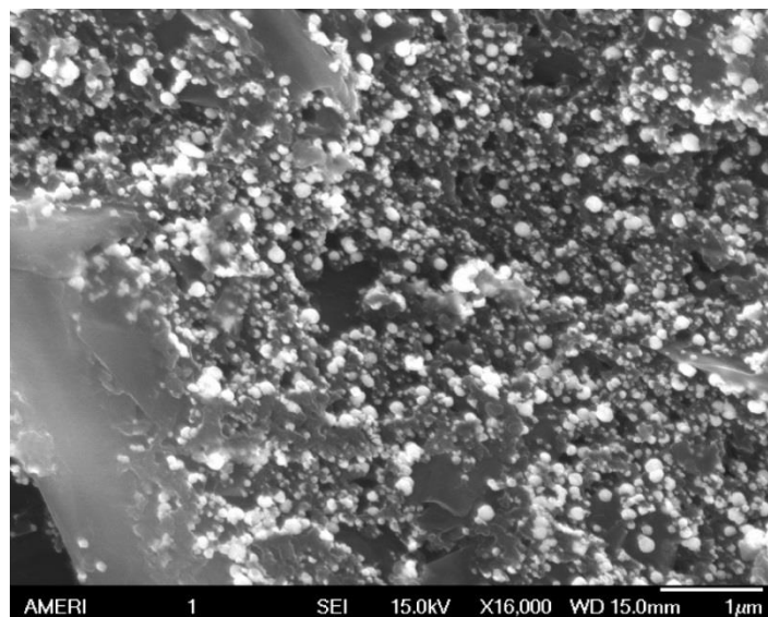
Figure 15: SEM image of the copper Oxide Nanoparticle deposited SPCE. The Particle size ranges from ~150nm.
