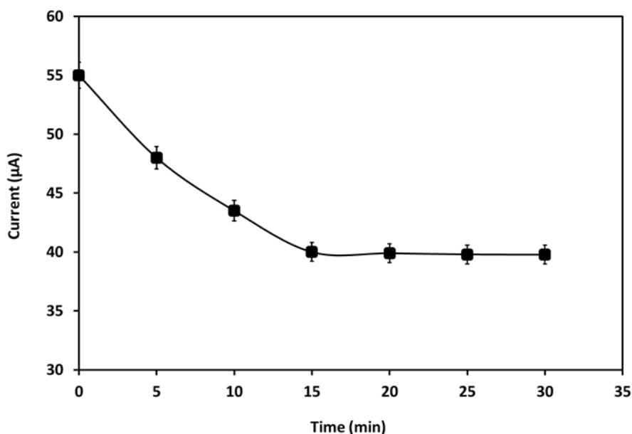
Figure 29: Effect of incubation time on current response of the cortisol MIP
