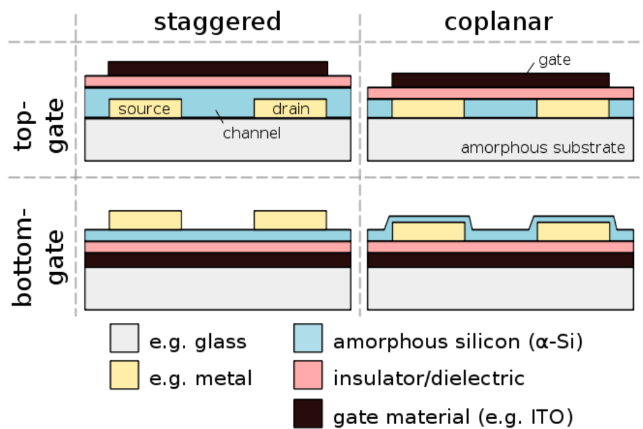
Figure 8: Different configurations of a TFT [1]
