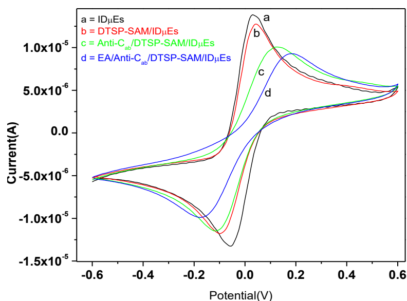
Figure 9: CV studies of IDEs (a) DTSP-SAM modified IDEs (b), Anti-Cab immobilized DTSP-SAM/IDEs electrode (c), and EA immobilized Anti-Cab/DTSP-SAM/IDEs immunoelectrode (d) using 5 \mu L PBS (pH 7.4) containing 5 mM [Fe(CV)6]3-/4- at 50 mV/s.
