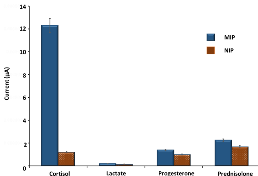
Figure 30: The change in peak current values observed at cortisol MIP (blue) and NIP (red) electrode in the presence of cortisol and other interferents individually each at 100 nM.
