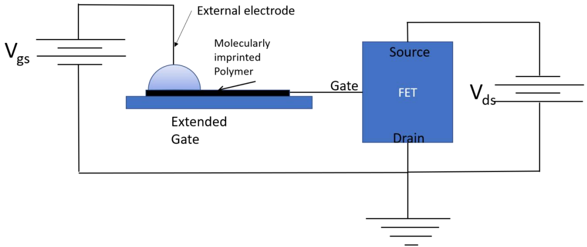
Figure 33: Scheme of the EGFET - MIP based sensing system
