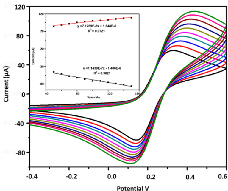
Figure 28: CV studies of the cortisol MIP sensor as a function of scan rate (50-150 mV/s), inset: magnitude of current response vs. scan rate.
