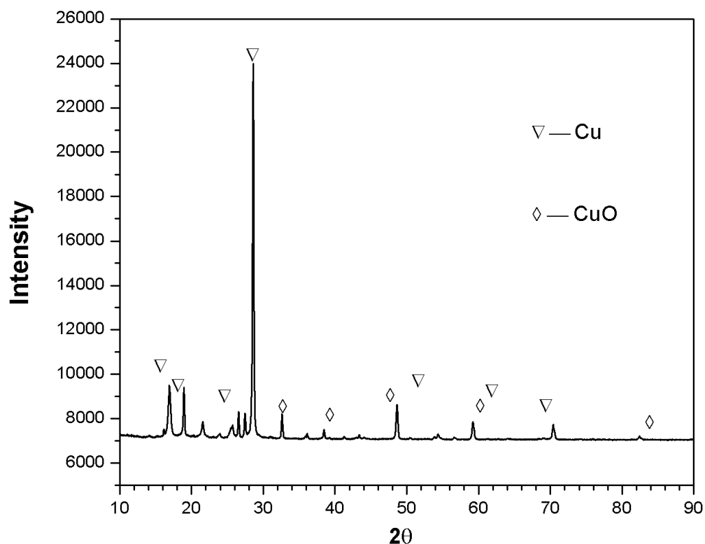
Figure 16: XRD image of Copper/ Copper oxide nanoparticles on the SPCE
