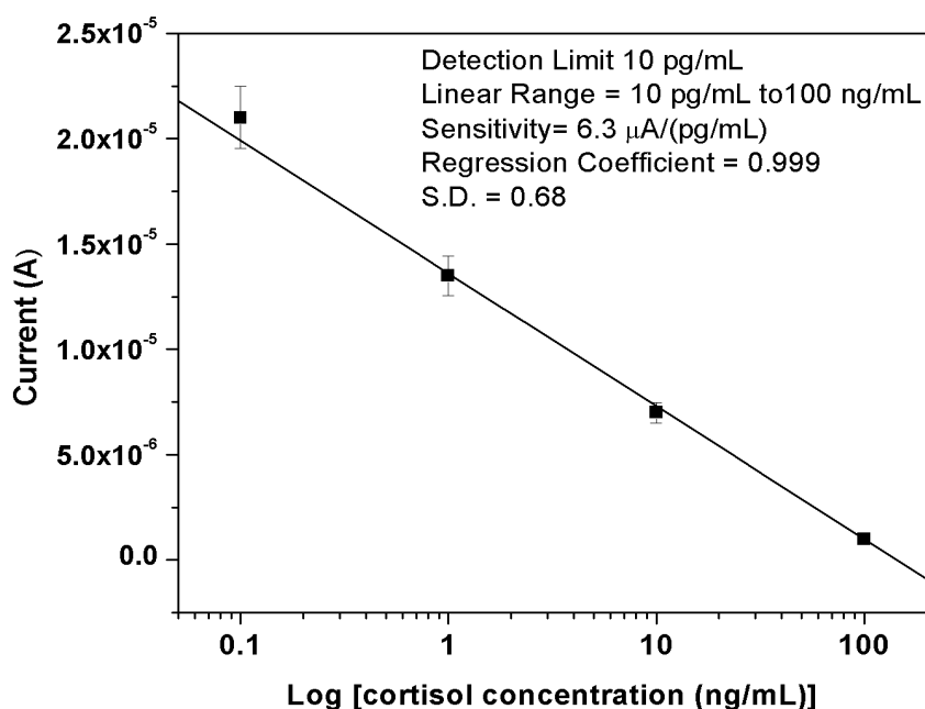
Figure 11: Calibration curve plotted between the magnitudes of current response obtained and logarithm of cortisol concentration (10 pg/mL to 100 ng/mL)
