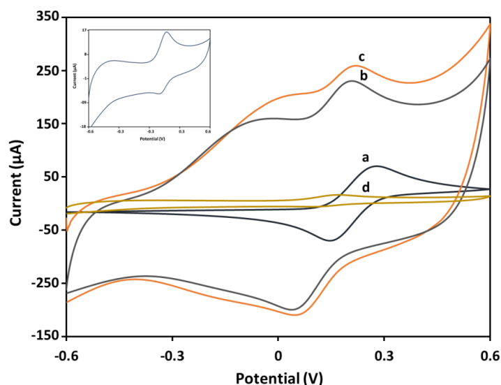
Figure 21: CV scans of 5 mM K 4 [Fe(CN) 6 ]/K 3 [Fe(CN) 6 ] solution at (a) bare SPCE, (b) PPy-SPCE, (c) Cortisol-PPy-SPCE and (d) MIP-PPy-SPCE; scan rate of 50 mVs -1 ; (Inset: Enlarged version of curve d).
