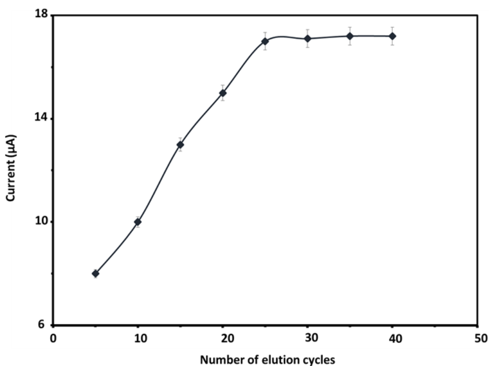
Figure 26: Effect of electrochemical extraction cycle on the current response
