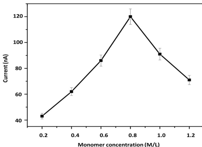
Figure 24: Effect of the monomer concentration on the response of the sensor to cortisol
