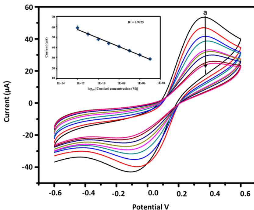
Figure 31: Electrochemical response studies of MIP-PPy-SPCE as a function of cortisol concentration (1 pM to 10 \mu M) using five mM K_4[Fe(CN)_6]/K_3[Fe(CN)_6] solution, inset: calibration curve between the magnitude of response current and logarithm of cortisol concentration
