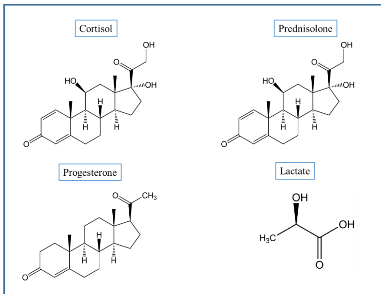
Figure 32: Molecular structure of cortisol and its structural analogs prednisolone, progesterone and lactate.
