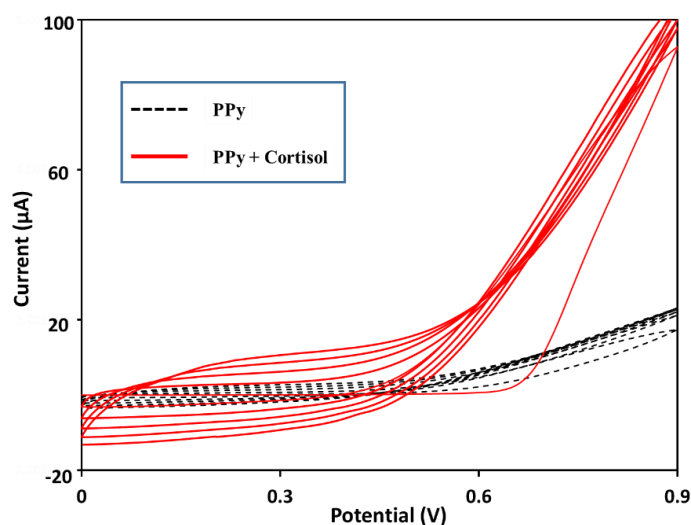
Figure 19: CV scans taken during the electropolymerization of pyrrole in the absence (dotted lines) and in the presence (solid lines) of 10 mM cortisol onto the SPCE. Scan rate: 50 mV/s.
