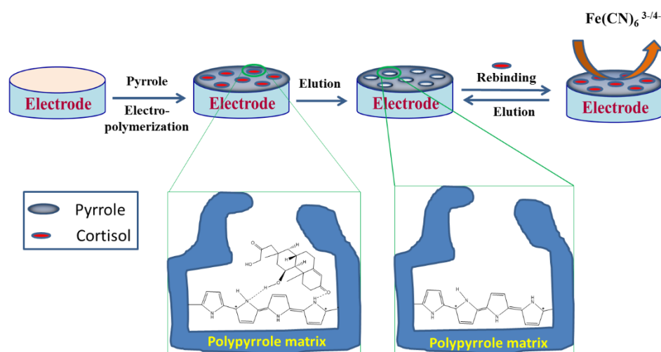
Figure 6: Schematic for fabrication of cortisol MIP biosensor on SPCE surface.
