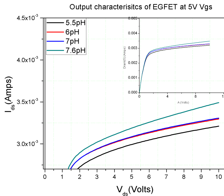
Figure 34: current response of the EGFET after the addition of PBS at different pH Values.
