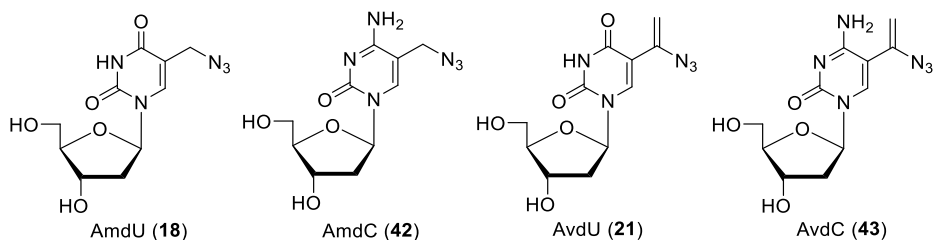
Figure 14. 2'-Deoxyuridine and 2'-deoxycytidine with azidomethyl and azidovinyl modified at C5
