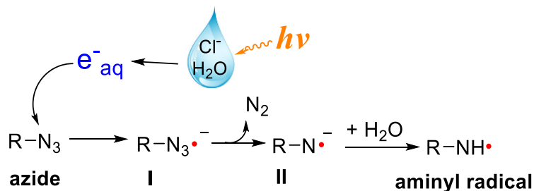
Scheme 3. The mechanism of formation of aminyl radicals on electron attachment to azido compounds in \gamma -irradiated aqueous glassy system
