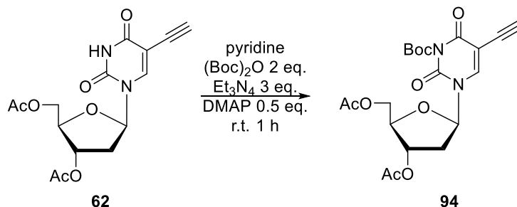
Scheme 25. Synthesis of 3- N -Boc-3',5'-di- O -acetyl-5-ethynyl-2'-deoxyuridine 94
