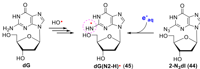
Figure 15. A plausible generation of 2'-deoxyguanosin-N2-yl radical (dG(N2-H)•) from 2-azido-2'-deoxyinosine
