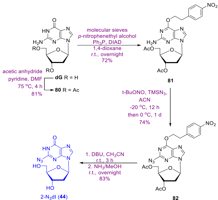
Scheme 23. Synthesis of 2-azido-2'-deoxyinosine
