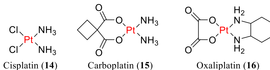
Figure 4. Platinum analogues applied clinically as a radiosensitizers
