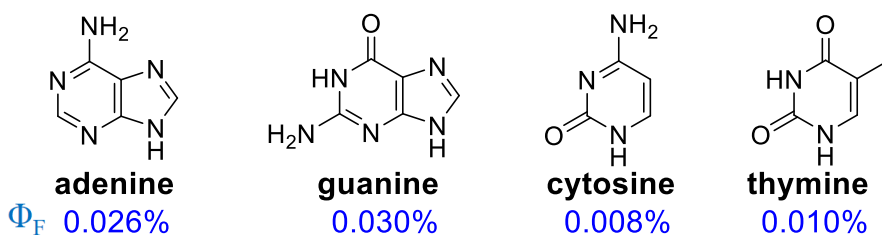
Figure 8. Fluorescence of the natural purine and pyrimidine bases
