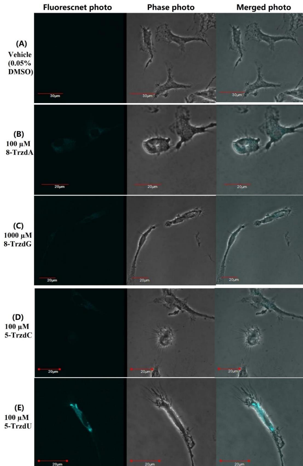
Figure 30. Fluorescence microscopy images and phase photos of primary mouse astrocytes cells treated with 8-TrzdA, 8-TrzdG, 5-TrzdC, and 5-TrzdU
