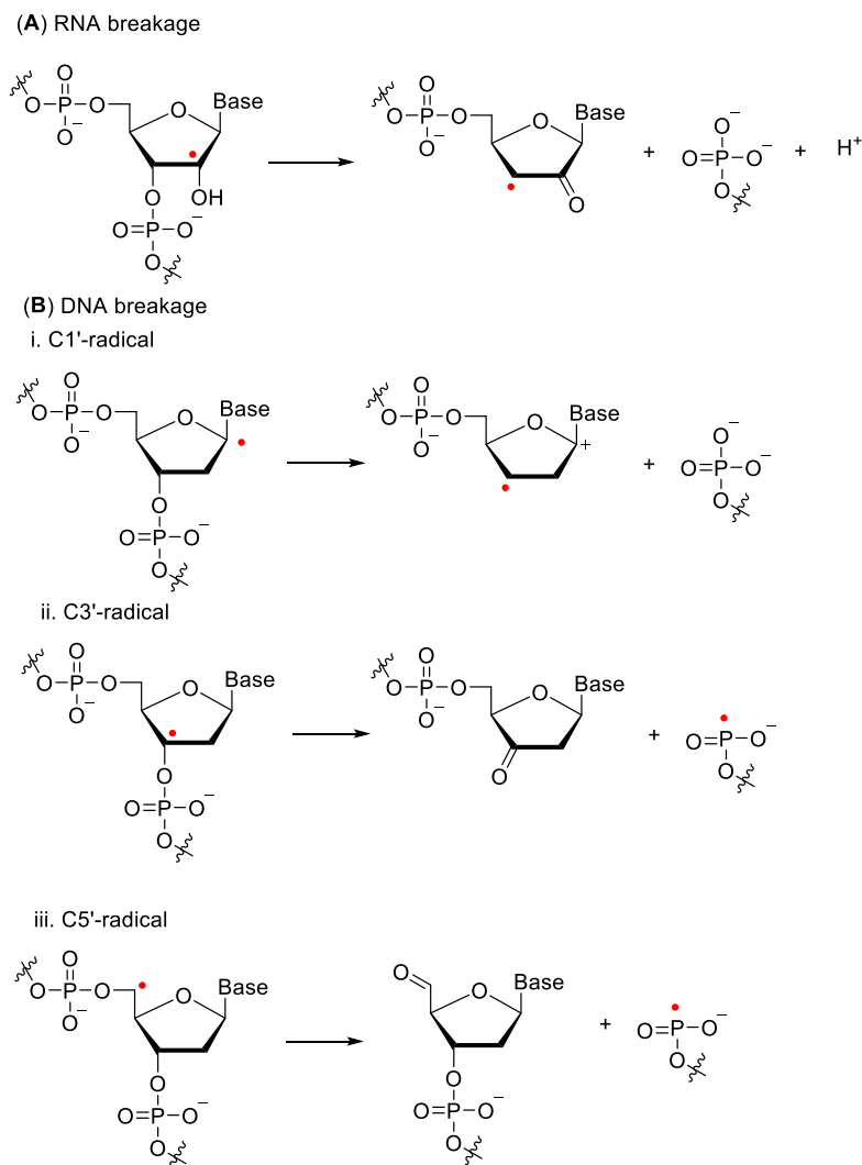
Scheme 6. Mechanism of RNA/DNA single-strand breaks upon generation of sugar radicals
