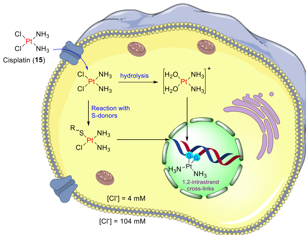
Figure 5. Mechanism of the anticancer activity of cisplatin
