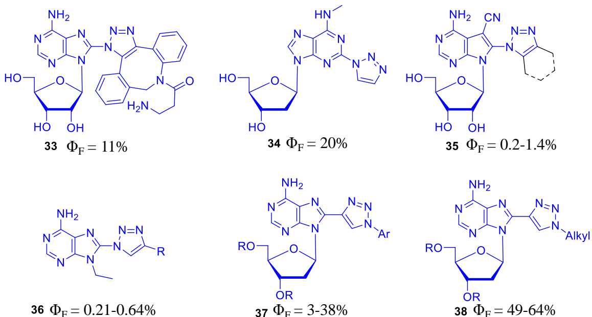
Figure 12. Structure and the fluorescent properties of N -substituted triazoles
