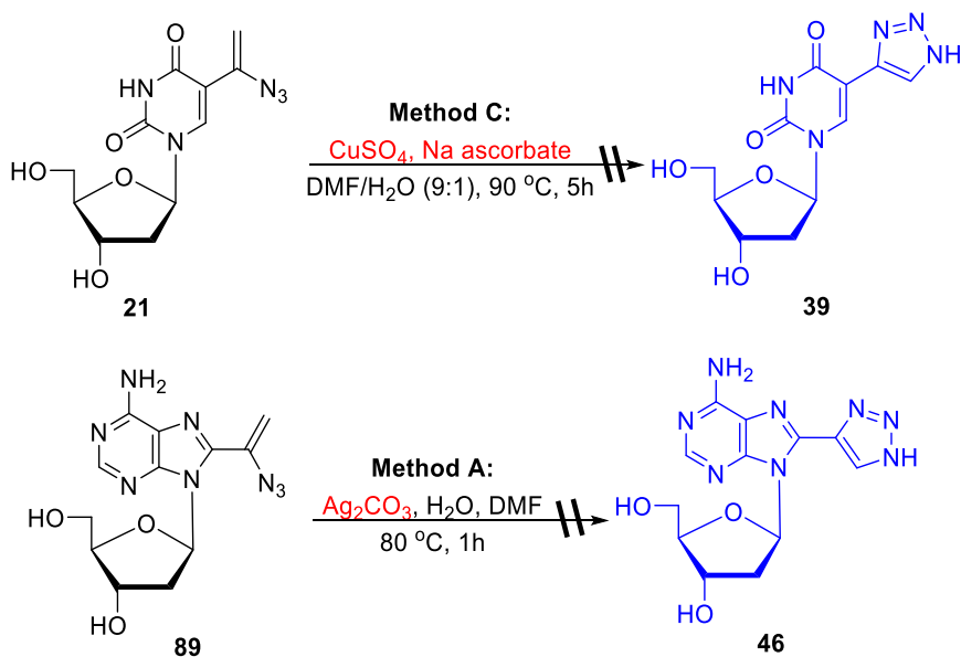
Scheme 26. Attempted conversion of vinylazides to triazoles
