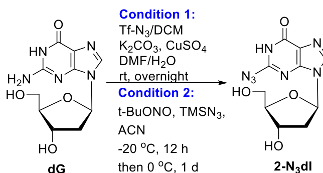
Scheme 22. Attempted one-step synthesis of 2-azido-2'-deoxyinosine
