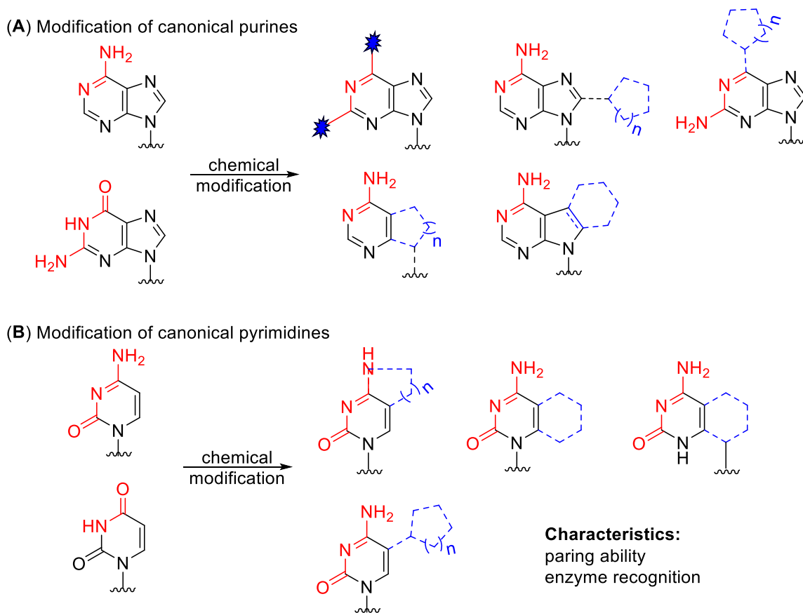
Figure 9. Canonical fluorescent nucleobase analogues
