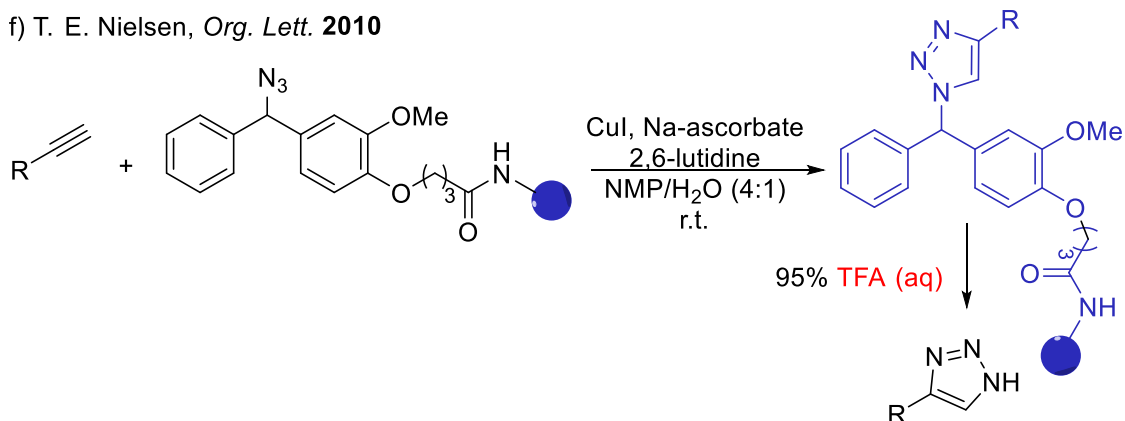
Scheme 9. Reported strategies for the synthesis of N -unsubstituted triazoles
