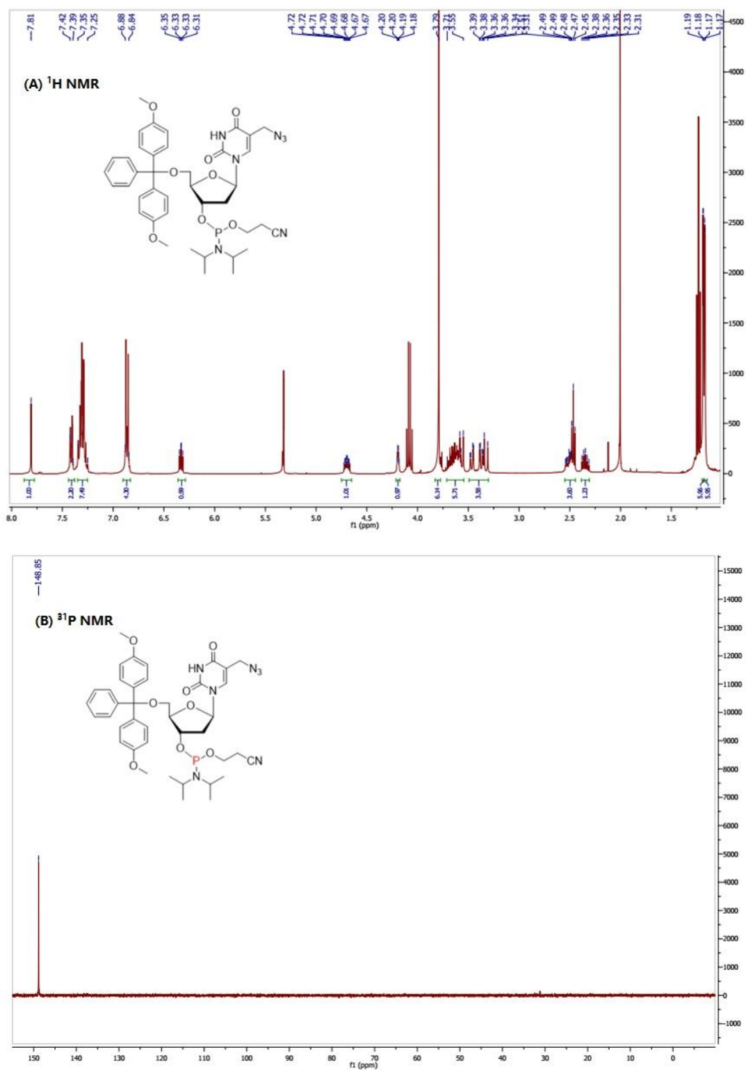
Figure 18. ^1\text{H} (A) and ^{31}\text{P} (B) NMR spectra of AmdU phosphoramidite 60 single diastereomer
