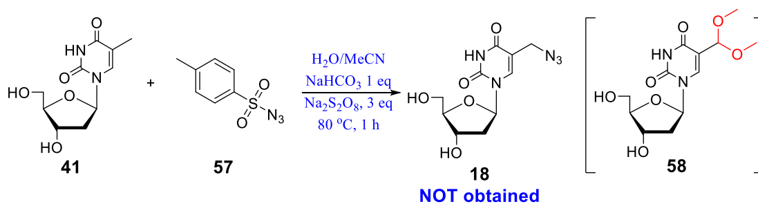
Scheme 11. Attempted one-step synthesis of AmdU
