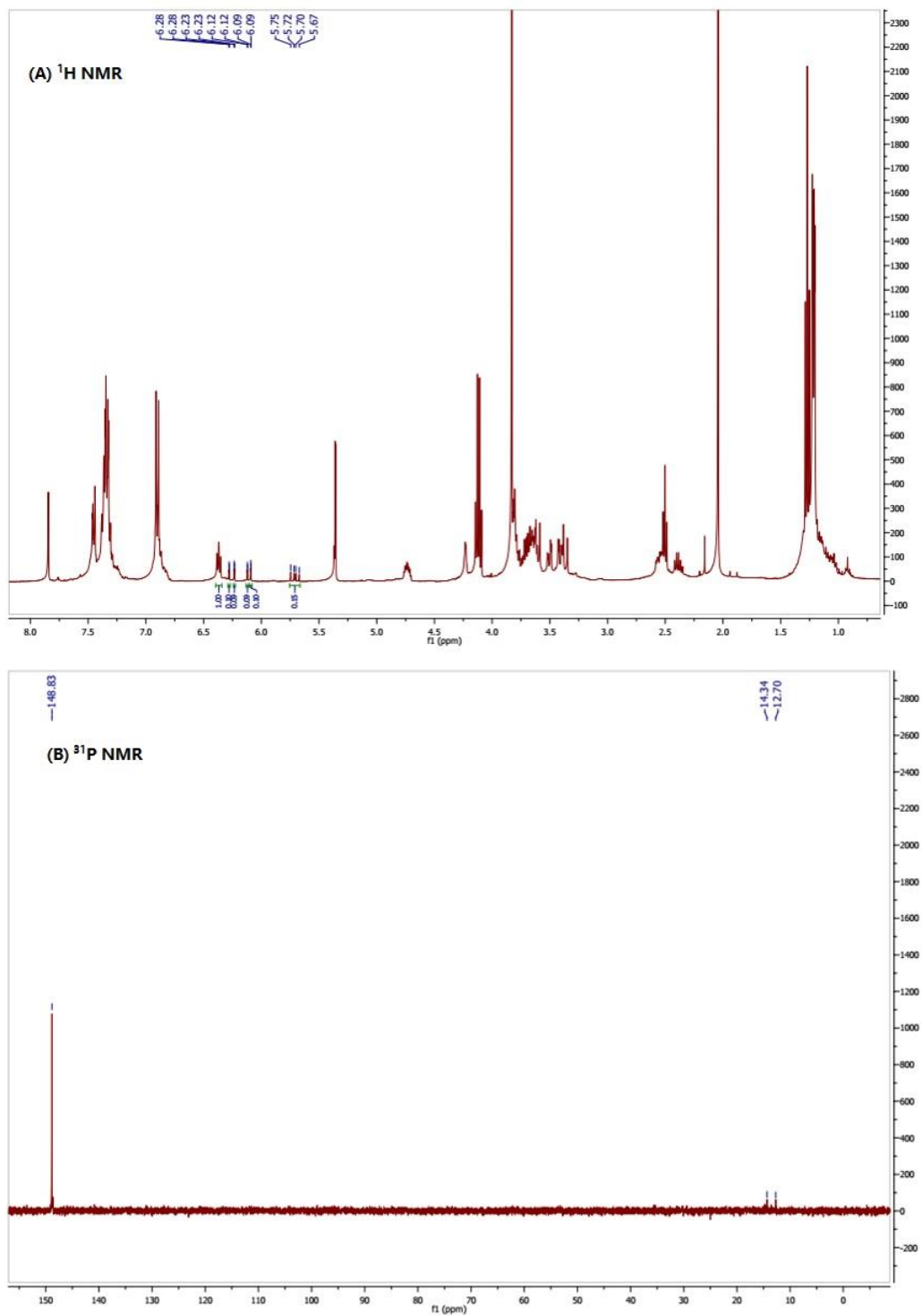
Figure 19. ^1\text{H} (A) and ^{31}\text{P} (B) NMR spectra showing decomposition of phosphoramidite 60 (in \text{CD}_2\text{Cl}_2 at room temperature for 15 h)
