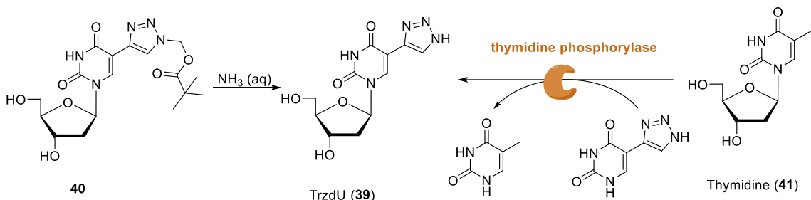
Scheme 8. Strategies for the synthesis of 5-TrzdU
