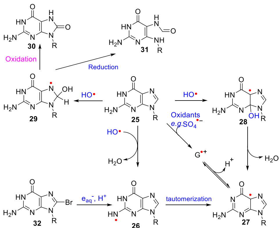
Scheme 7. Radical reactions of guanine with hydroxyl radicals and subsequent reactions
