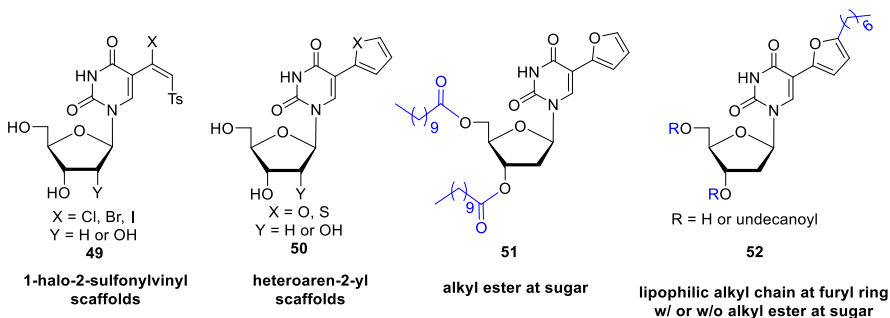
Figure 17. 5-(1-Halo-2-sulfonylvinylyl) and 5-(2-furyl) uracil nucleosides prodrugs
