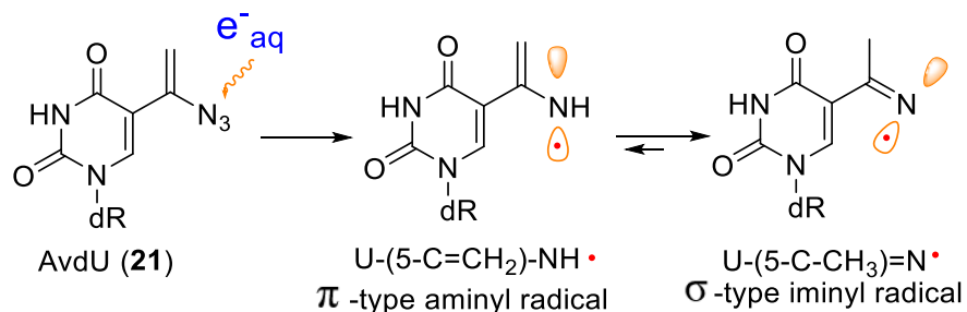
Scheme 21. Tautomerization of the \pi -type aminyl radical generated from AvdU 21 to the \sigma -type iminyl radical
