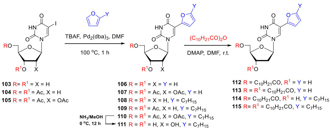
Scheme 29. Synthesis of 5-(fur-2-yl)- or 5-(5-heptylfur-2-yl)uracil nucleosides by direct C-H arylation
