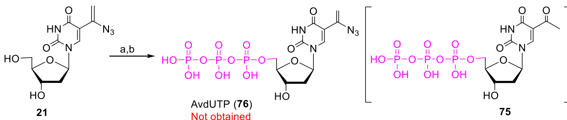
Scheme 18. Attempted synthesis of AvdUTP 76
