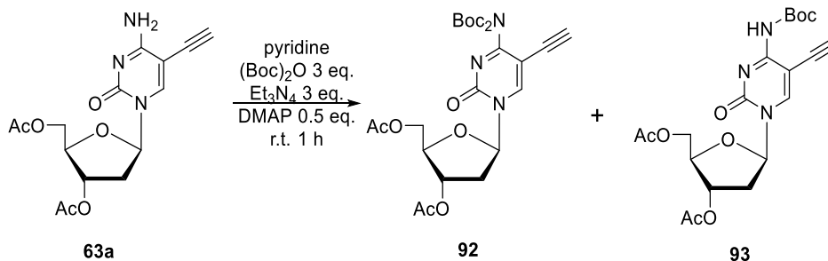
Scheme 24. Synthesis of 4- N -Boc protected 3',5'-di- O -acetyl-5-ethynyl-2'-deoxycytidine derivatives 92 and 93
