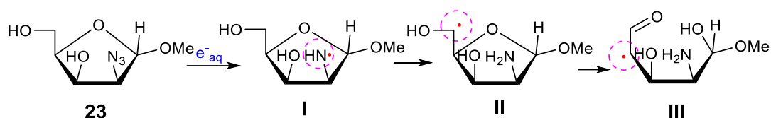
Scheme 4. Formation of aminyl radicals in methyl 2-azido-2-deoxy- \alpha -D-lyxofuranoside and subsequent intramolecular H-atom transfer and ring opening
