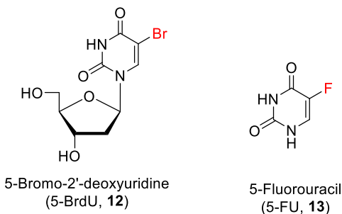
Figure 3. Structures of C5 halogenated pyrimidine bases and nucleosides
