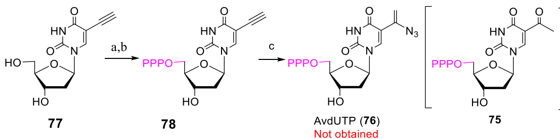
Scheme 18. Attempted synthesis of AvdUTP 76
