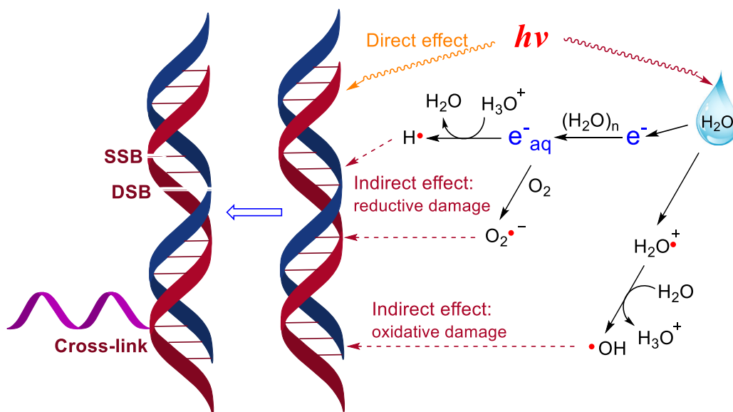
Scheme 1. The rationale for the direct/indirect effects of irradiation in radiotherapy
