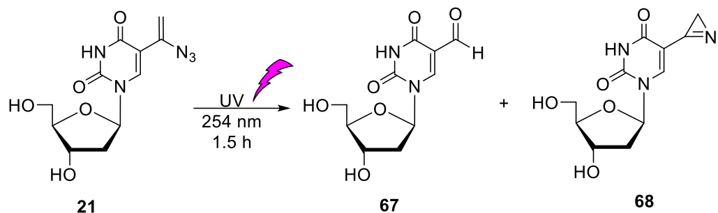
Scheme 14. Decomposition of AvdU under 254 nm UV
