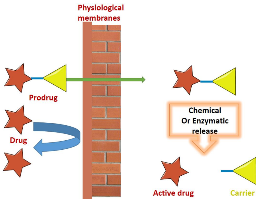
Figure 13. A simplified illustration of the prodrug concept
