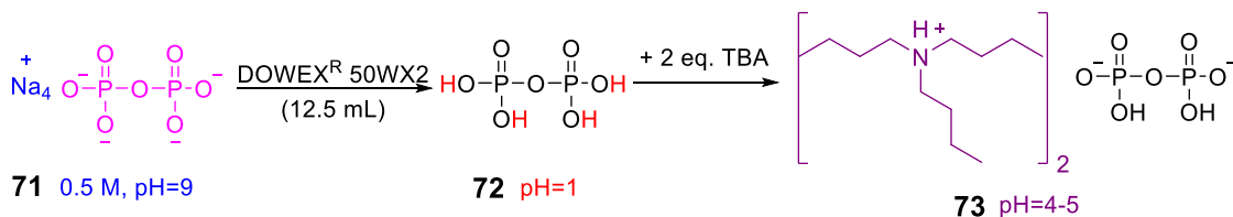
Scheme 16. Preparation of tributylammonium pyrophosphate (TBAPP)
