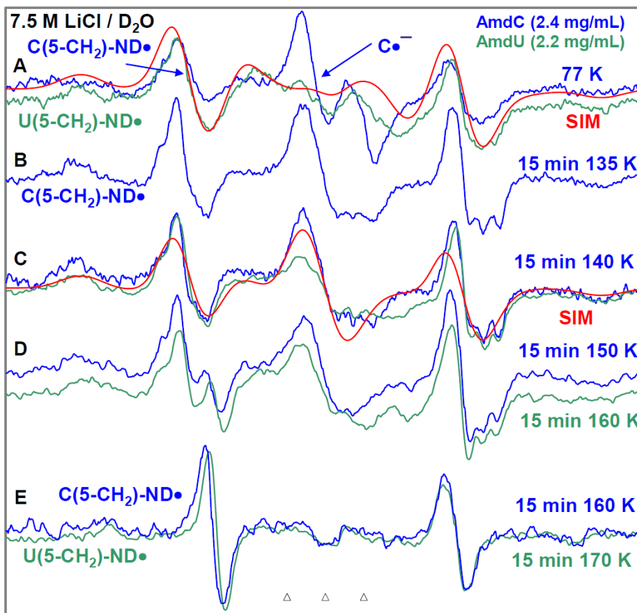
Figure 25. ESR spectra of AmdC after radiation-produced prehydrated one-electron attachment at 77 K and stepwise annealing as well as simulated spectra. Spectra (A-D) were obtained from AmdC 42 (2.4 mg/mL) by subtraction of 250 G \text{Cl}_2\cdot^- spectrum from the individual experimentally recorded spectrum. (A) ESR spectrum (blue) after radiation-produced prehydrated one-electron addition to AmdC at 77 K in 7.5 M LiCl/D 2 O. Spectra (B, blue) to (E, blue) were obtained from the same sample of 7 via stepwise annealing of the sample for 15 min at 134, 140, 150 and at 160 K. All spectra were recorded at 77 K. The experimental spectra from AmdU 18 (2.2 mg/mL, sea-green) are superimposed in (A), (C), (D), and (E) for comparison. The red spectra in (A) and in (E) are the simulated spectra.
