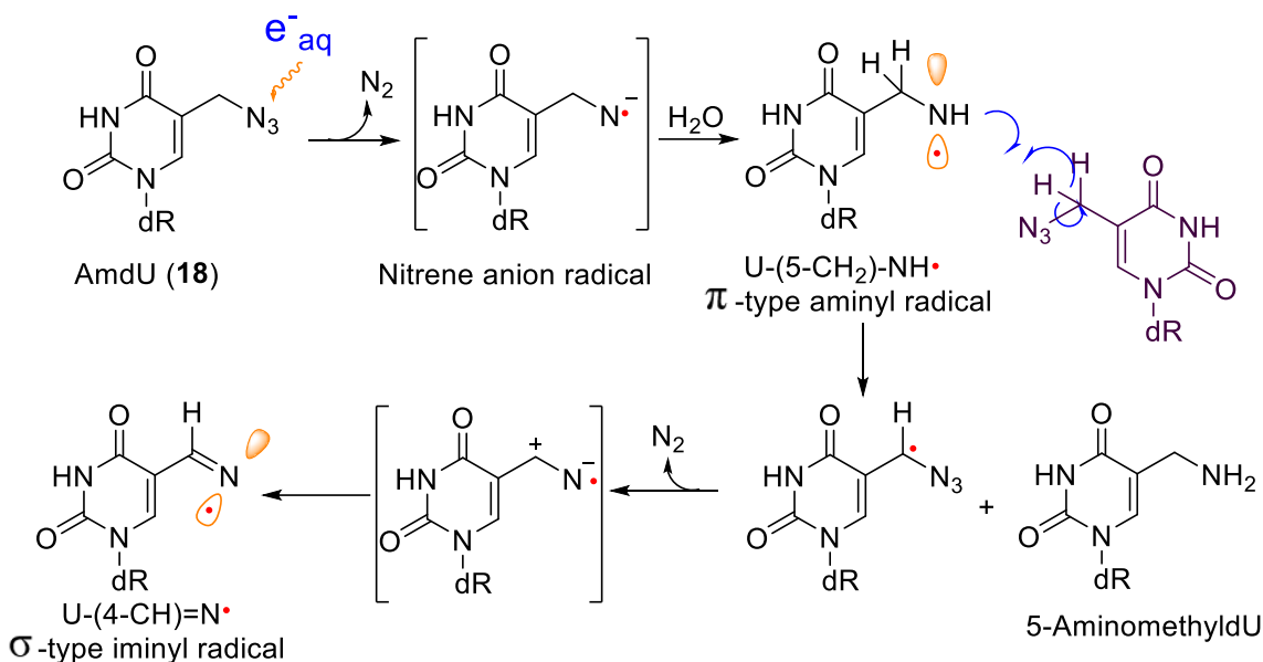
Scheme 20. Formation of \pi -type aminyl radical from AmdU 18 and its bimolecular conversion to the \sigma -type iminyl radical
