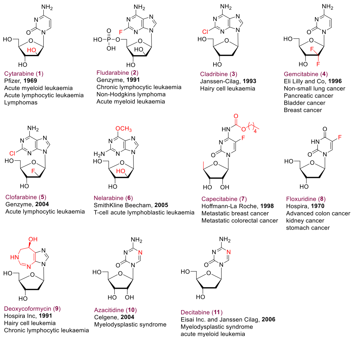
Figure 1. Approved anticancer nucleoside/tide drugs
