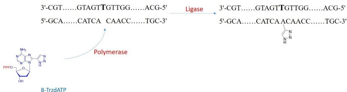
Figure 33. Proposed incorporation of 8-TrzdATP into DNA
