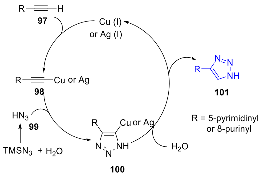
Scheme 27. Mechanism for the formation of N -unsubstituted 1,2,3-triazoles
