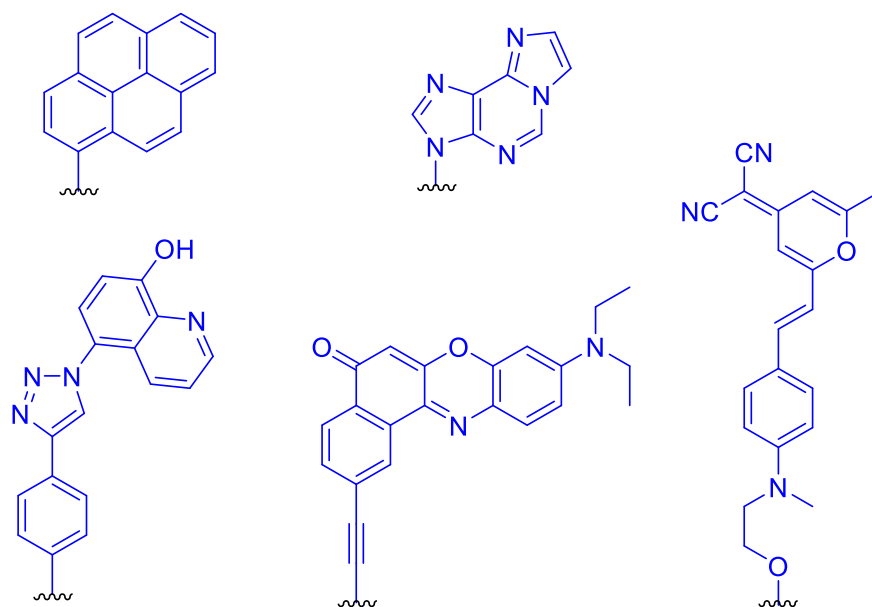
Figure 10. Non-canonical fluorescent nucleobases
