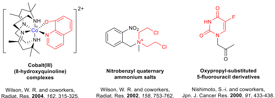
Figure 6. Radiosensitizers activated by irradiation-induced prehydrated electron
