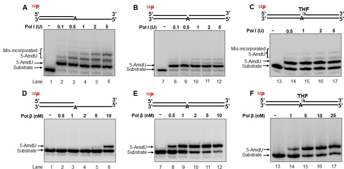
Figure 20. Incorporation of AmdUTP 20 into duplex DNA by pol I and pol \beta . Measurement of incorporation of an AmdUTP by Klenow fragment on the open template (A) and one-nucleotide gap substrate (B), and the one-nucleotide gap substrate containing a 5'-THF at the downstream strand (C). Measurement of incorporation of an AmdUTP by pol \beta on the open template (D) and one-nucleotide gap substrate (E), and substrate containing a 5'-THF at the downstream strand (F). Lanes 1, 7, and 13 represent substrate only. Lanes 2-6, 8-12, and 14-17 represent the products resulting from incorporation of an AmdUTP.
