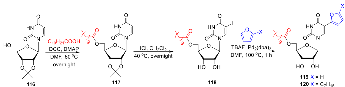
Scheme 30. Synthesis of 5-(fur-2-yl)- or 5-(5-heptylfur-2-yl)uridine and their 5'-esters
