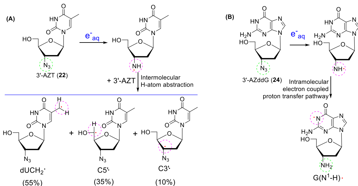
Scheme 5. Prehydrated one-electron attachment to azido group on 3'-AZT(A) and 3'-AZddG (B): Aminyl radical formation and subsequent reactions
