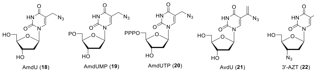
Figure 7. Azido-modified pyrimidine nucleoside/tide analogues
