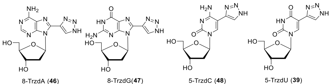
Figure 16. Fluorescent N -unsubstituted 1,2,3-triazol-4-yl nucleosides
