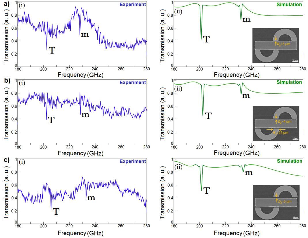
Figure 7.6. Normalized transmission amplitude profiles of the THz resonator system with three different offset gaps obtained (i) experimentally and (ii) numerically for (a) D_g=3\ \mu\text{m} , (b) D_g=4\ \mu\text{m} , and (c) D_g=5\ \mu\text{m} . The insets are the SEM images with the geometrical parameters.
