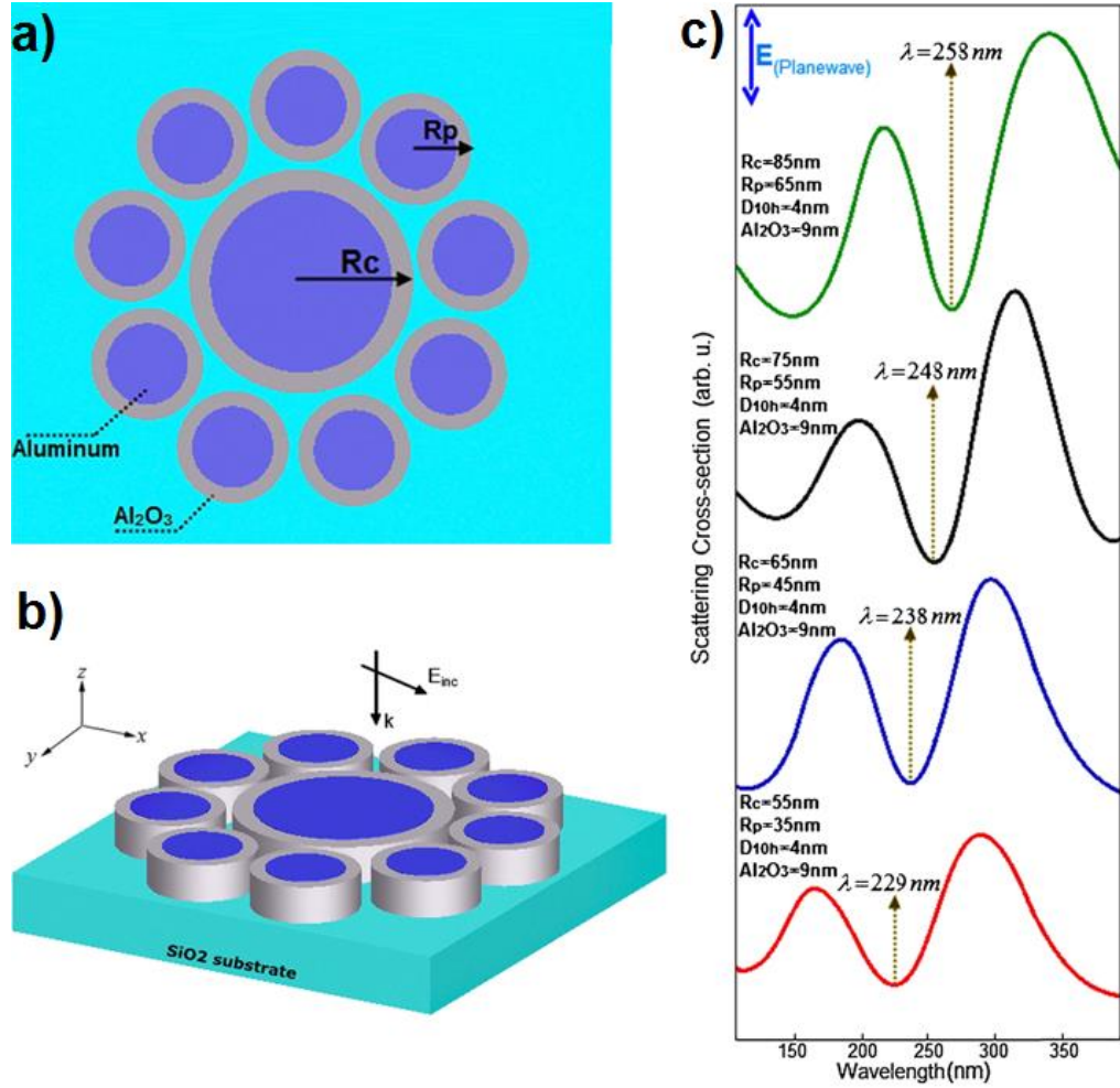
Figure 3.11. Plasmonic Response of an Al decamer. a) and b) Schematics of the Al decamer with a coverage of oxide layer around nanodisks. c) Scattering cross-section for different geometrical variations.
