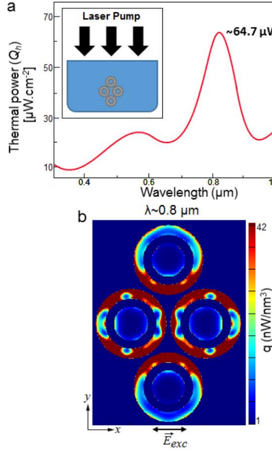
Figure 6.2. a) Thermal heat power flux ( Q_h ) profile for a metallic nanoassembly during laser pump exposure in a liquid system. b) Dissipated power density mapping in a metallic quadramer at the peak of absorption.
