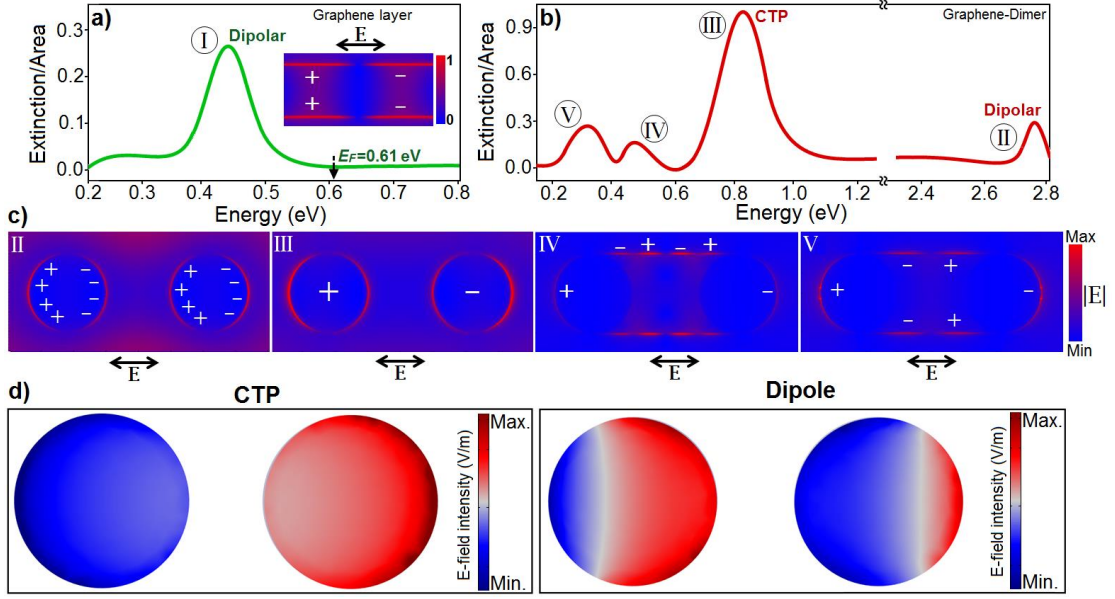
Figure 4.11. a) Extinction cross-section of a highly-doped to E_F = 0.61 eV ( n -type) graphene nanoribbon under optical excitation at room-temperature T = 300 K. The inset is the E-field intensity map for the dipolar mode. b) Extinction spectra of plasmonic nanodimer antenna on the highly doped graphene nanoribbon bridge, supporting dipolar (II), CTP (III), quadrupolar (IV), and dipolar (V) moments. c) The local |E| -field intensity snapshots for the plasmon resonance excitation and distribution across the device for dipole (II) and CTP (III) modes. d) The charge density plots for the CTP spectral feature and dipolar modes.
