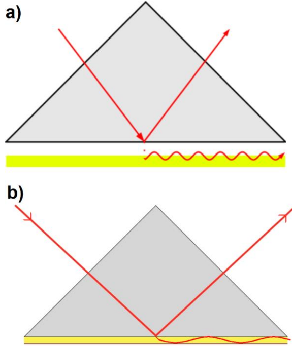
Figure 2.3. SPR excitation setups. a) Otto configuration, b) Kretschmann configuration.
