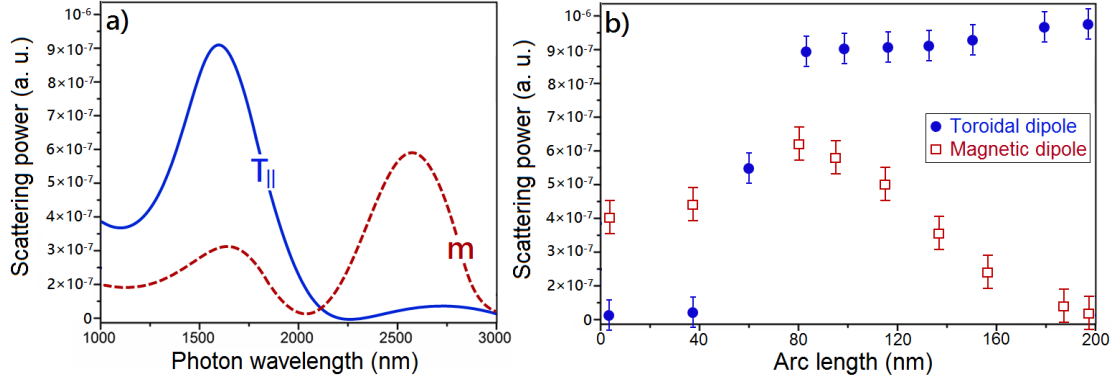
Figure 5.9. a) Scattering powers of toroidal and magnetic moments ( L_{arc} ). (b) The scattering power as a function of arc length variations for toroidal and magnetic moments.
