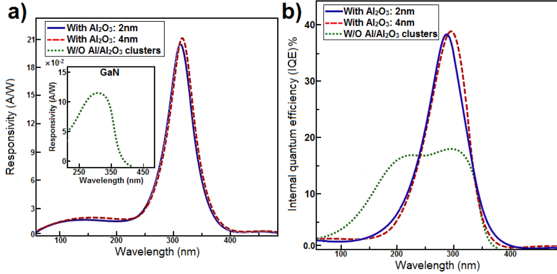
Figure 3.20. The spectral responses for the UV detector in both non-plasmonic and plasmonic regimes, with variant Al 2 O 3 thicknesses of heptamer clusters. a) Responsivity profile under 5.0 V applied bias. Inset is the responsivity profile for the non-plasmonic regime. b) The IQEs for different regimes of the UV detector.
