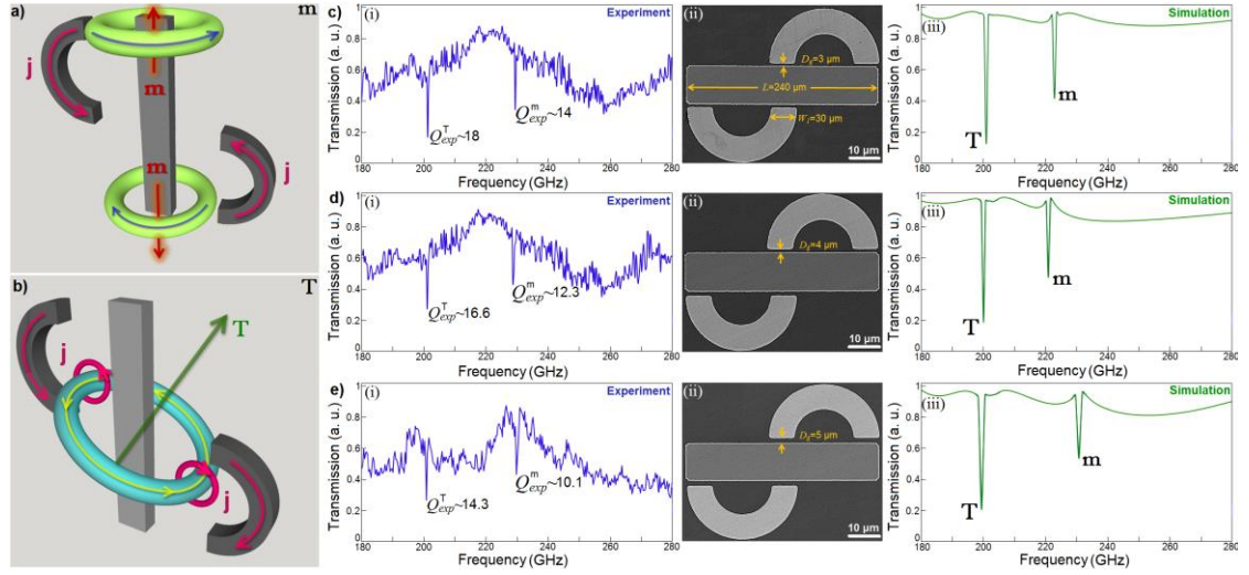
Figure 7.4. a) and b) The 3D schematics of the magnetic (m) and toroidal (T) resonances around and across the central and surrounding magnetic resonators, respectively. c), d), and e) The electromagnetic response of the compositional THz plasmonic resonator: (i) Experimentally obtained normalized transmission amplitude profiles for the unit cells with three different offset gaps, (ii) the SEM images for different offset gaps between resonators, (iii) Numerically calculated transmission spectra for three different offset gaps.
