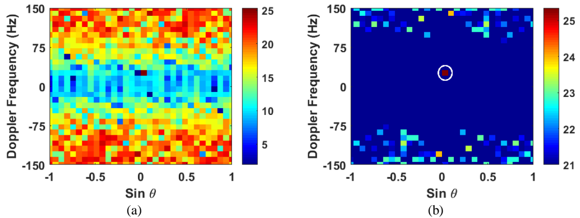
Figure 3.13 Clutter removal result for Example 2 when moving platform effects are compensated perfectly. (a) Before denoising processing; (b) after denoising processing.
