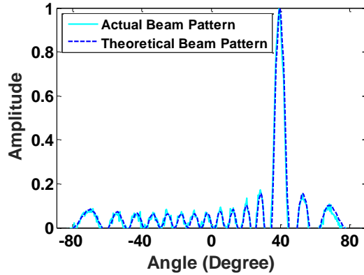
Figure 5.7 Refocused transmit-receive beam pattern with mainlobe pointing in 40°.
