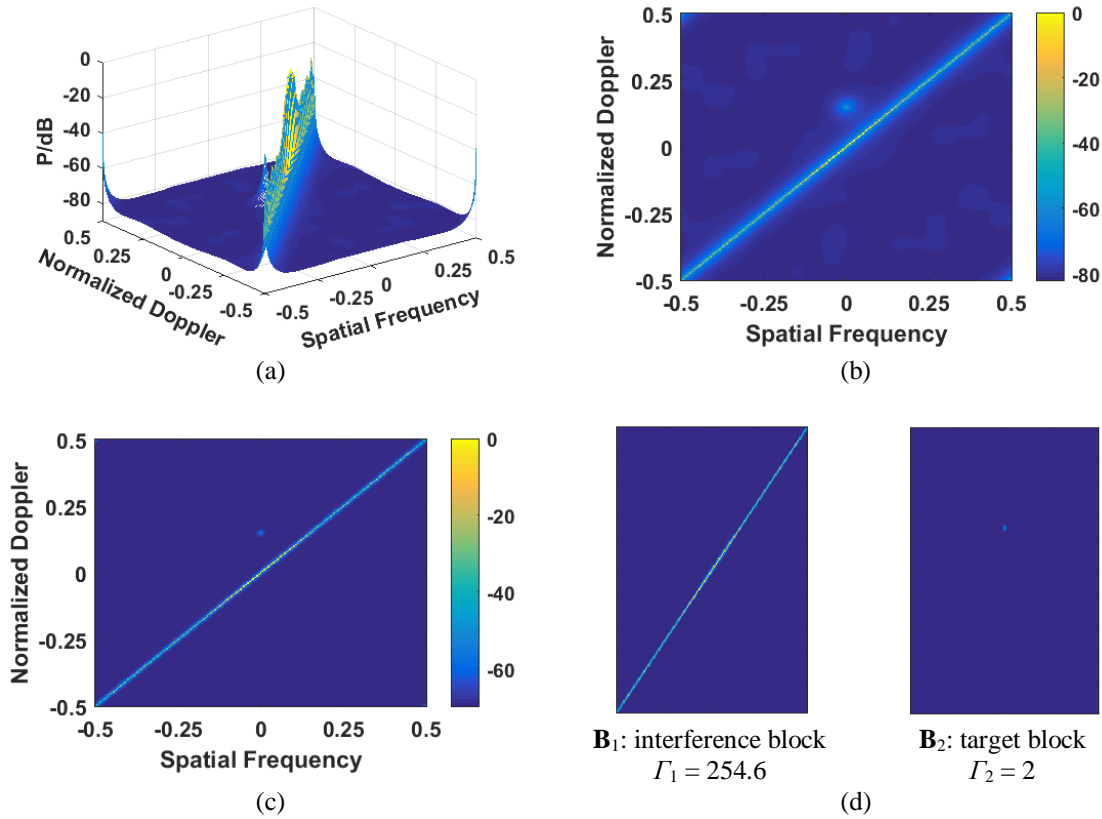
Figure 2.11 BDIFR processing results for Example 5.
