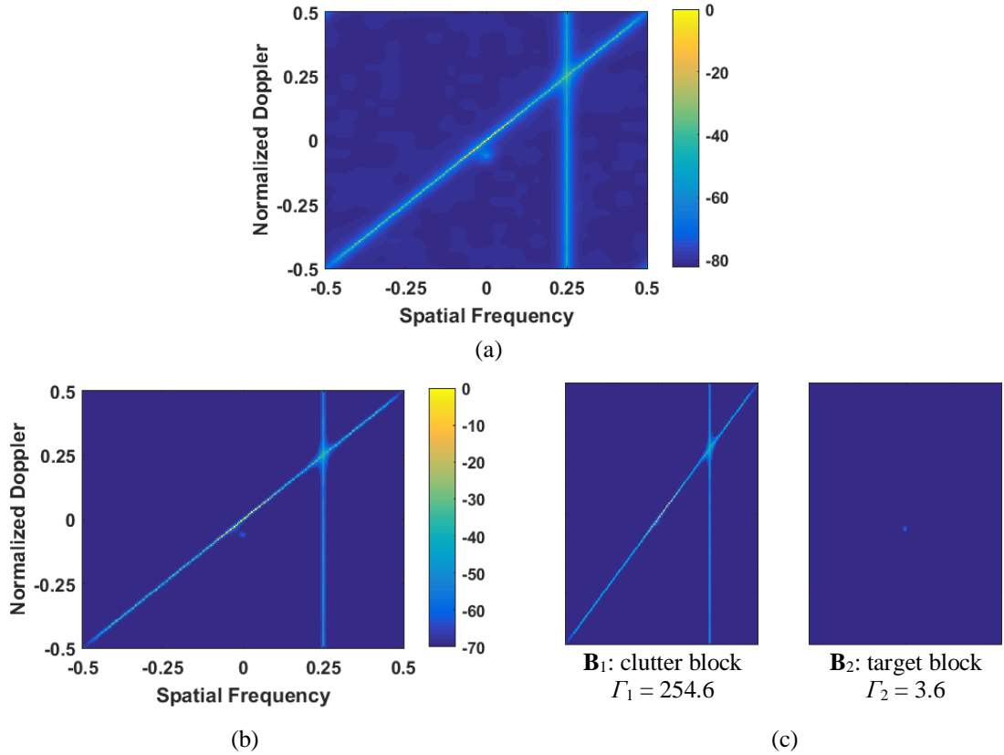
Figure 2.14 BDIFR processing results for Example 8.
