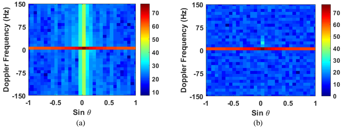
Figure 3.11 Doppler compensation result for Example 2.
