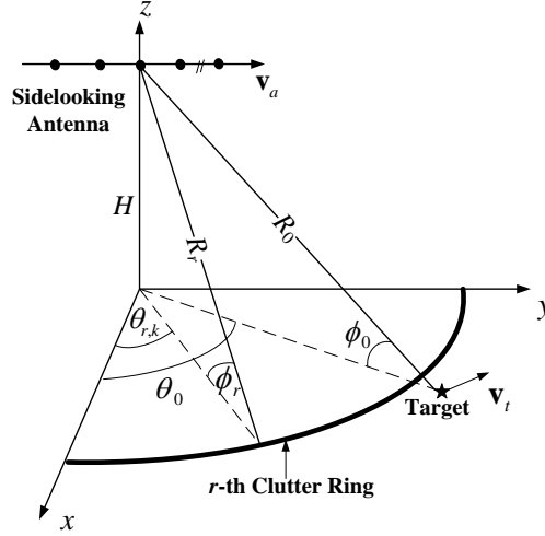
Figure 2.2 Airborne radar platform geometry.
