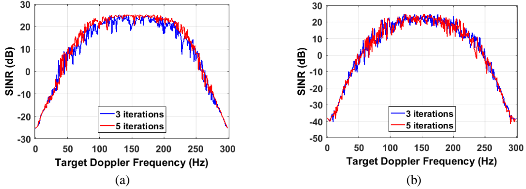
Figure 4.16 SINR performances for different number of iterations. (a) MIMO radar with 1 st -RSTAP (b) MIMO radar with 2 nd -RSTAP.
