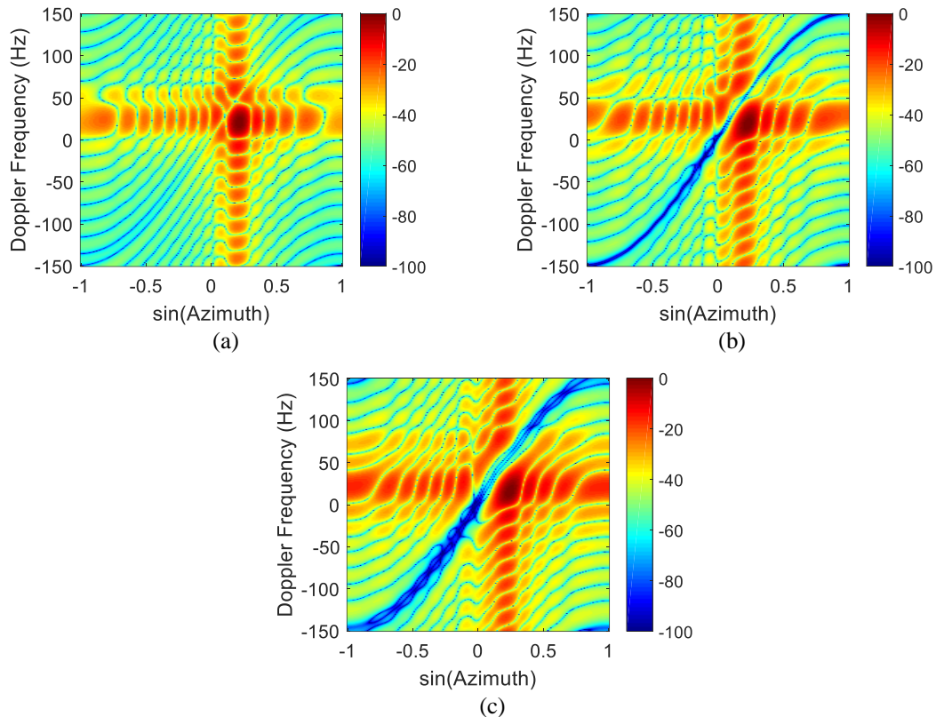
Figure 4.5 2D angle-Doppler responses for different spectral spread values when conventional STAP filter is used (phased-array radar).
