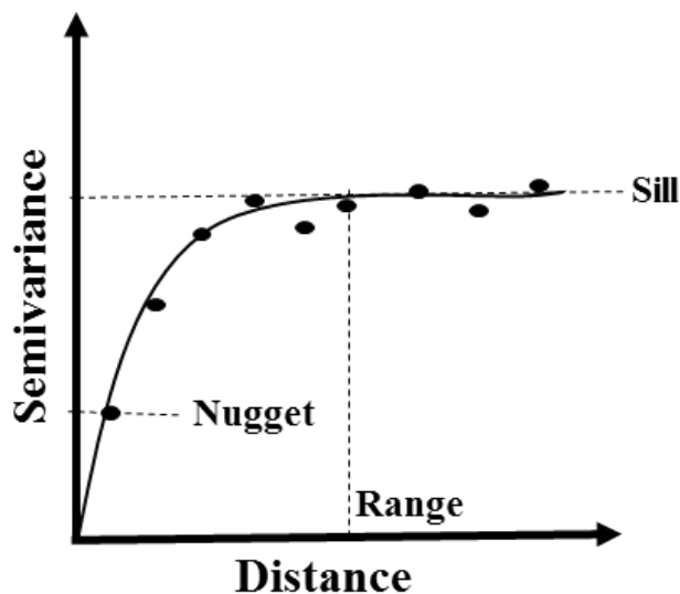
Figure 2. The semivariograms show the hypothetically observed distance class (filled circles) and the fitted model (solid line). The theoretical semivariogram model fitting is usually expressed by three parameters: nugget, sill, and range. The nugget represents the measurement errors or spatial dependence at scales not explicitly sampled. The sill represents the variance of the correlated measurements. The range shows the extent of heterogeneity (i.e., zone of influence or distance of dependence) [9,53].
