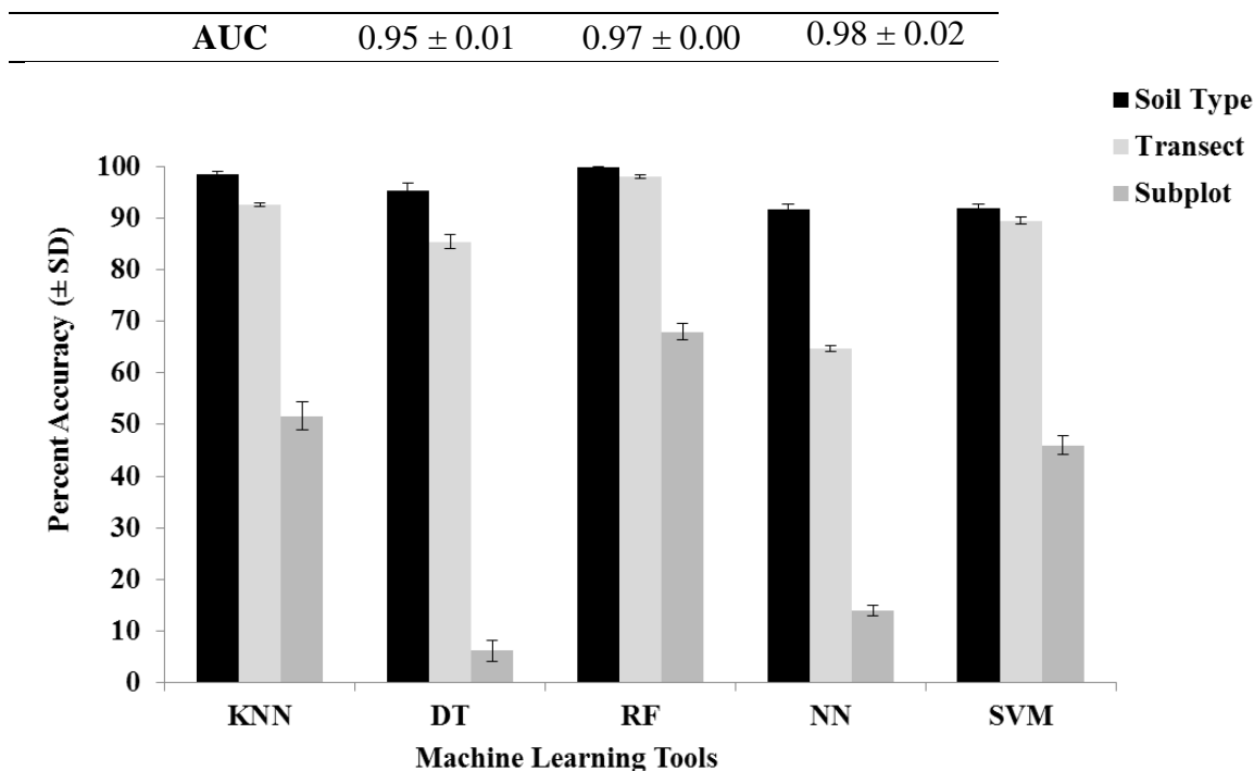
Figure 5. Prediction accuracy values and AUC values ( \pm SD of the mean) for each of the five machine learning tools (KNN, DT, RF, NN, SVM) using training and test sets randomly chosen three different times from the complete database. Black bars = soil type, light grey bars = transect, dark grey bars = subplot.
