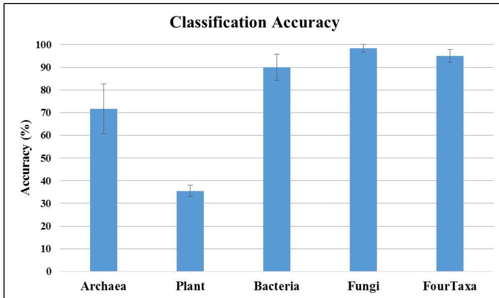
Figure 9. Random Forest classification accuracy using individual taxa and four-taxa to discriminate three sites (FIU, CC6, and KK). Archaea, bacteria, fungi, and four-taxa did not show a significant difference in classification accuracy ( p > 0.07 ).
