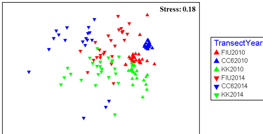
Figure 10. Temporal variability within three sites (Red=FIU, Blue=CC6, and Green=KK) across a four year time-span ( \blacktriangle 2010/ \blacktriangledown 2014) based on Nonmetric Multidimensional Scaling (nMDS) analysis using Bray-Curtis similarity coefficient.
