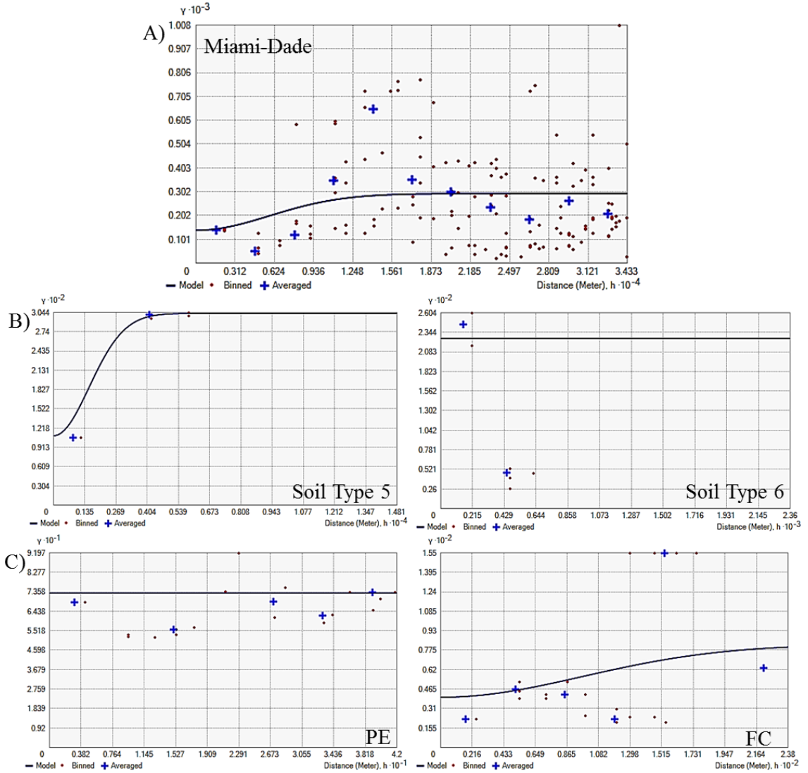
Figure 7. Semivariogram illustrating A) Miami-Dade spatial variability, B) soil type level spatial variability, C) Transect level variability.
