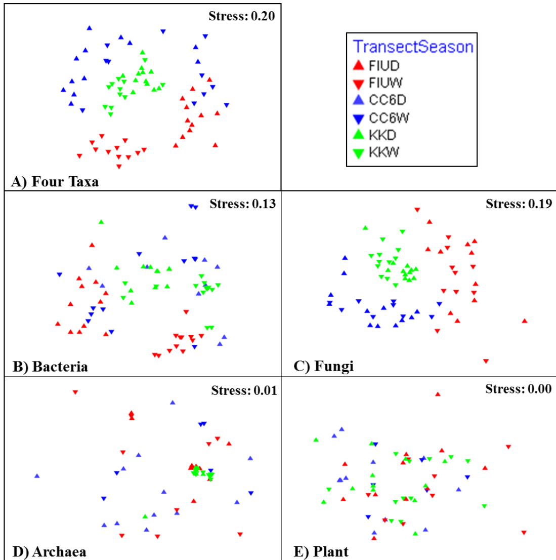
Figure 8. Nonmetric Multidimensional Scaling 2-D plots illustrating the discrimination power to distinguish three sites (Red=FIU, Blue= CC6, Green= KK) and season ( \blacktriangle Dry/ \blacktriangledown Wet). A) Four-taxa was able to discriminate sites and seasons within a site. B) Bacteria marker was able to group KK and group FIU based on season. C) Fungi was the best marker to discriminate the three sites. D) Archaea was unable to discriminate FIU and CC6; however, it was able to group KK. E) Plant was unable to distinguish the three soil sites apart.
