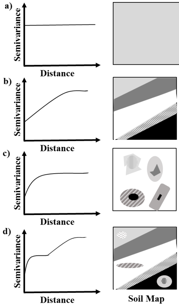
Figure 3. Plots illustrate different hypothetical semivariograms with their associated surface maps adapted from Ettema & Wardle (2002). A) pure nugget effect: no spatial structure was observed at the spatial extent studied. This can occur as a result of random sampling variance or variability that is occurring at other spatial scales not examined in the spatial extent. B) Large-scale heterogeneity: few, large and smoothly continuous gradients. C) Small-scale heterogeneity: many, small, sharply discontinuous patches. D) Nested heterogeneity: multiple scales of patchiness where more than one factor is influencing the pattern at different scales [9].
