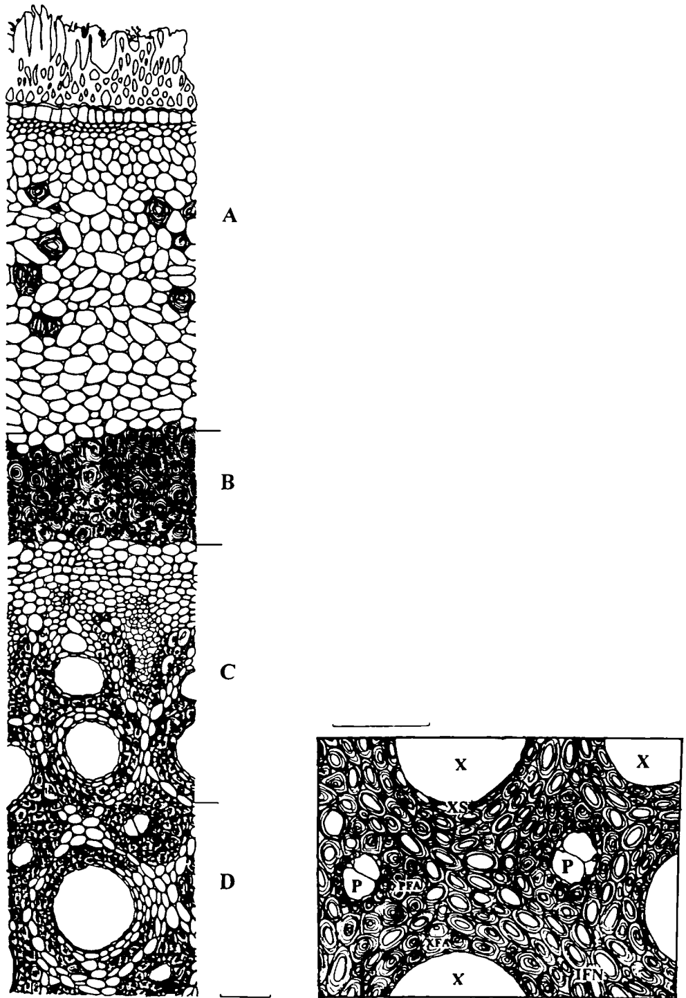
Figure 2.3 H. flexuosa absorbing root transverse-section including details of non-peripheral stele. Zone A = outer cortex; Zone B = circumstellar sclerenchymatous ring; Zone C = peripheral stele; Zone D = nonperipheral stele. X = xylem element; P = phloem element; XFA = xylem fiber aggregate; PFA = phloem fiber aggregate; XS = xylem sheath; IFN = Interfascicular network Scale bar = 100µm
