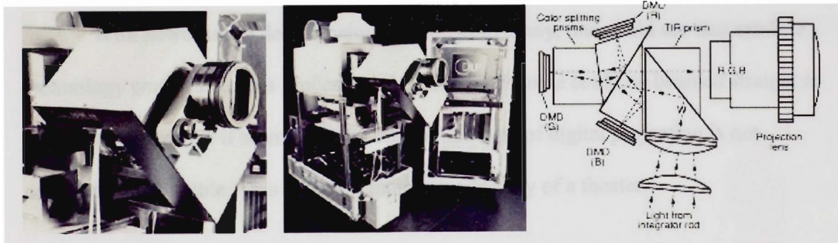
Figure26. (from Texas Instruments site www.spie.org/web/oer/march/mar99/micromirrors.html )
