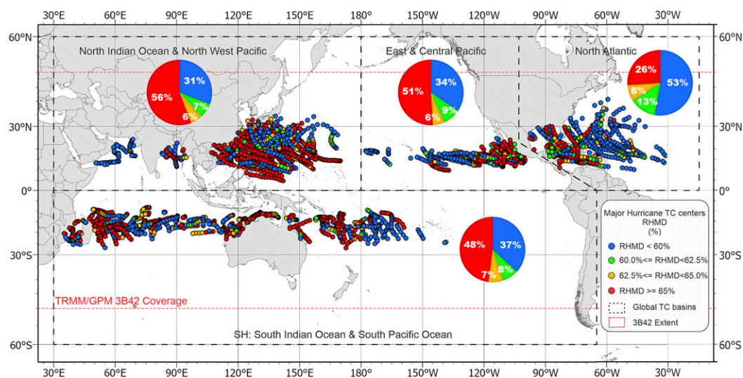
FIG. 10. Global map showing the locations of the centers of major hurricanes for each SHIPS data point categorized by different RHMD levels. Pie charts illustrate the percentage of observations for each RHMD category in each basin.
