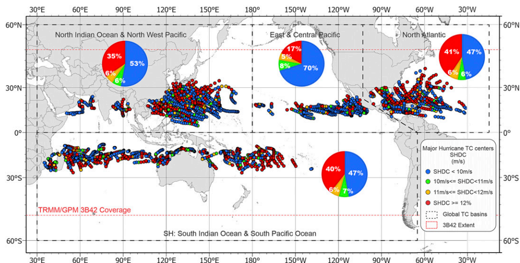
FIG. 11. Global map showing the locations of the centers of major hurricanes for each SHIPS data point categorized by different SHDC levels. Pie charts illustrate the percentage of observations for each SHDC category in each basin.
