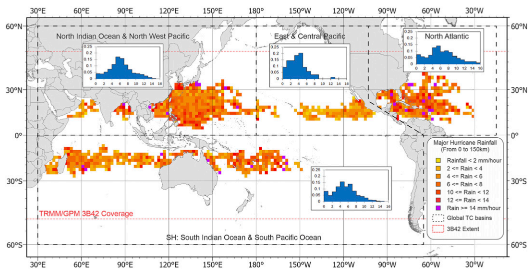
FIG. 7. Map showing the spatial distribution of the normalized TC rainfall produced by major hurricanes in the period 1998–2016 (only the inner-core region is considered). Pixel size is resampled to 2^\circ \times 2^\circ for better representation. Histograms show the normalized frequency of inner-core rainfall rate values for each basin.
