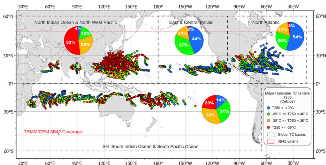
FIG. 12. Global map showing the locations of the centers of major hurricanes for each SHIPS data point categorized by different T250 levels. Pie charts illustrate the percentage of observations for each T250 category in each basin.
