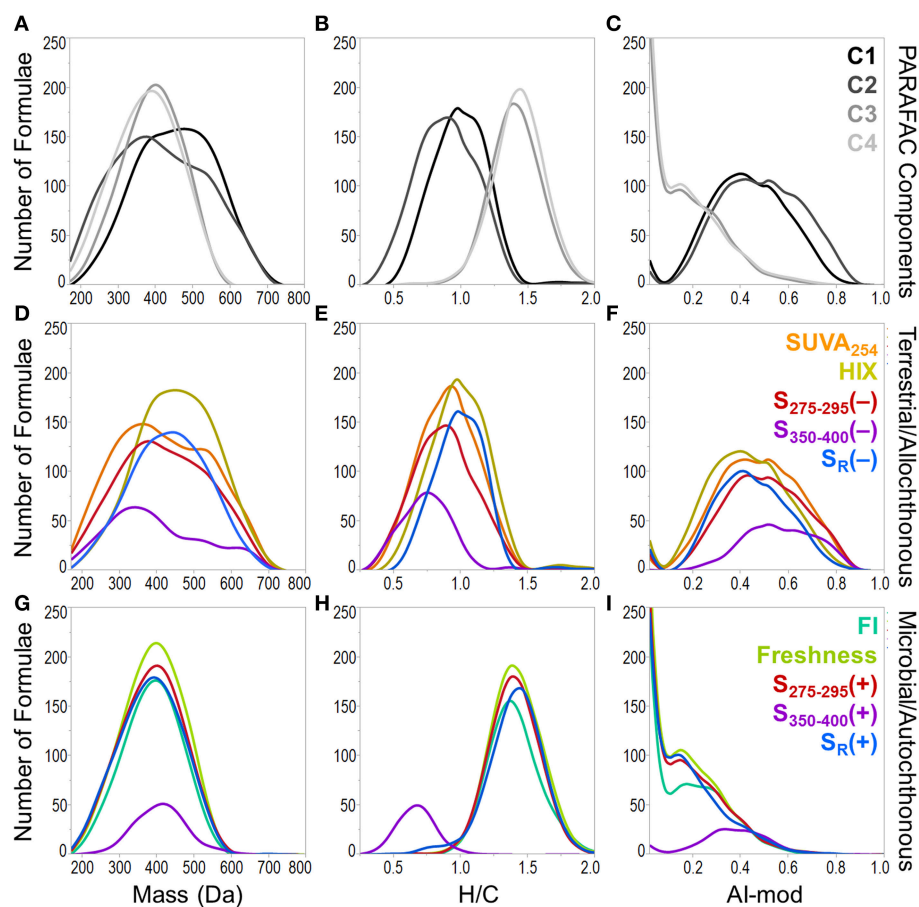
FIGURE 7 | Molecular mass (first column), H/C ratio (second column) and modified aromaticity index (AI-mod; third column) distributions of formulae associated with optical properties. Plots (A–C) show the distributions of formulae which positively correlated with PARAFAC components. Plots (D–F) show the distributions for optical properties which track with allochthonous or terrestrial-type DOM (formulae positively correlated with S_{UVA_{254}} , HIX and formulae negatively correlated with S_{275-295(-)} , S_{350-400(-)} , and S_R(-) ). Plots (G–I) show the distributions for optical properties which track with autochthonous or microbial-type DOM (formulae positively correlated with FI, freshness index, S_{275-295(+)} , S_{350-400(+)} , and S_R(+) ).
