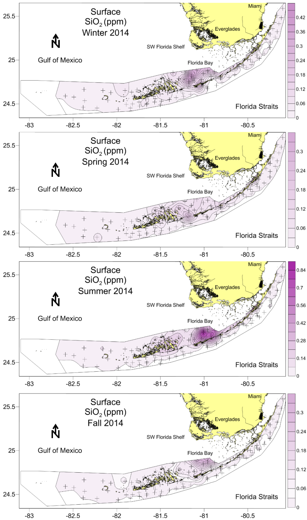
Figure 28. Distributions of surface silicate across the region during 2014.
