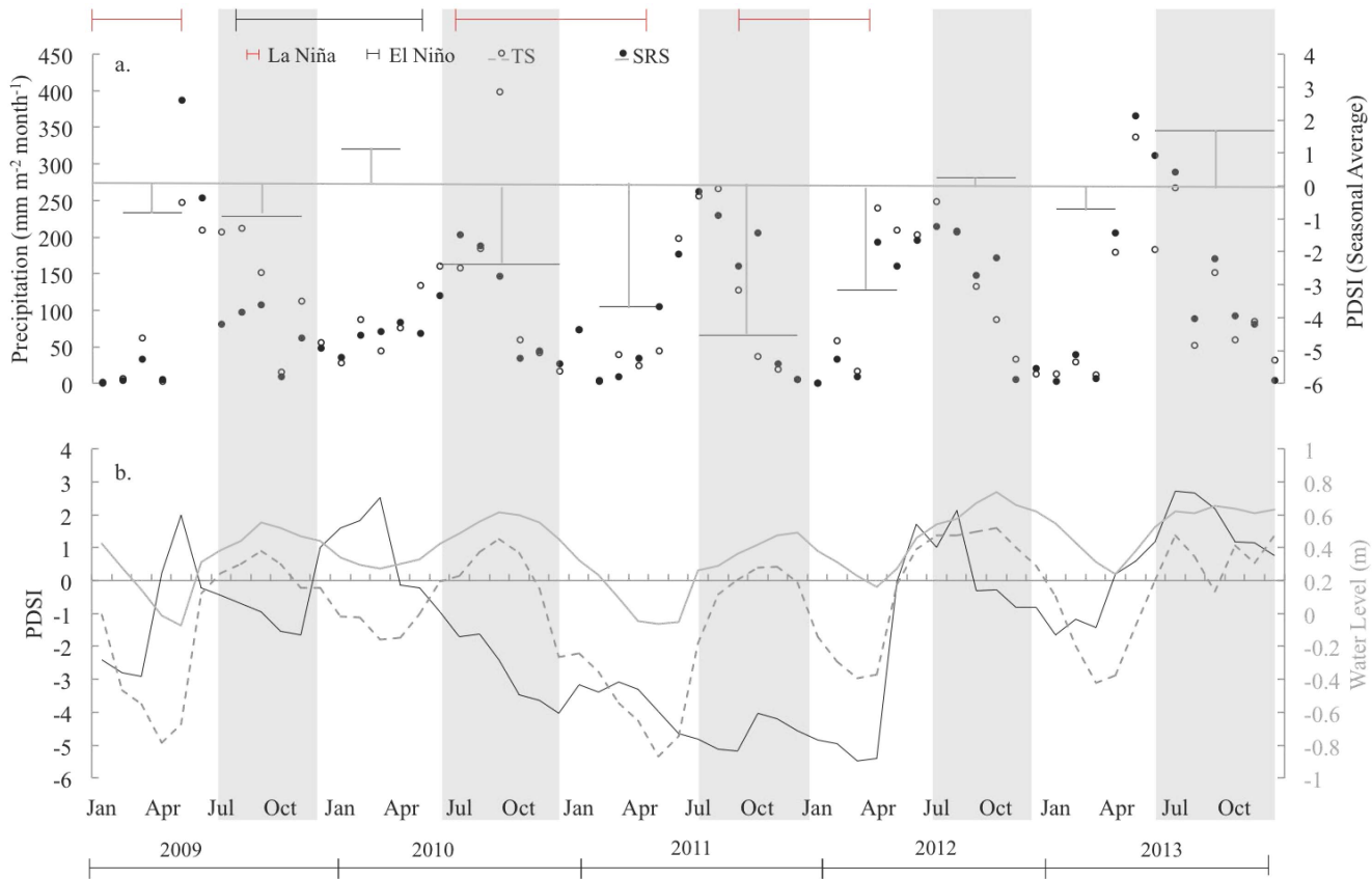
Fig 3. Time series of precipitation, PDSI, and water levels at TS and SRS. (a) Shows monthly cumulative precipitation (mm) and season intensity (as measured by seasonal average PDSI), (b) shows monthly average Palmer Drought Severity Index (PDSI), water level (m), and El Niño and La Niña phase.
