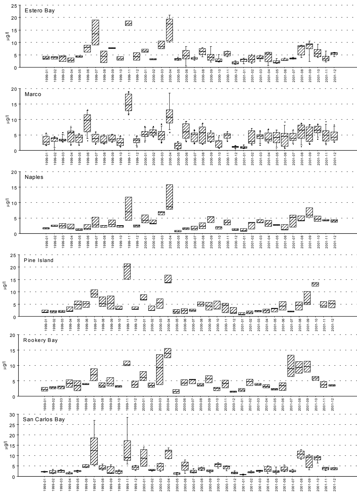
Figure 6.3. Monthly median and range of chlorophyll a in the Cape Romano-PIS area.
