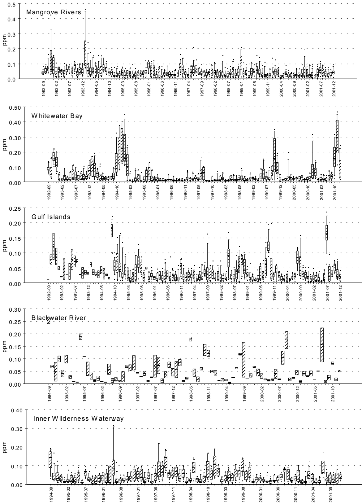
Figure 3.5. Monthly median and range of dissolved inorganic nitrogen in the five zones.
