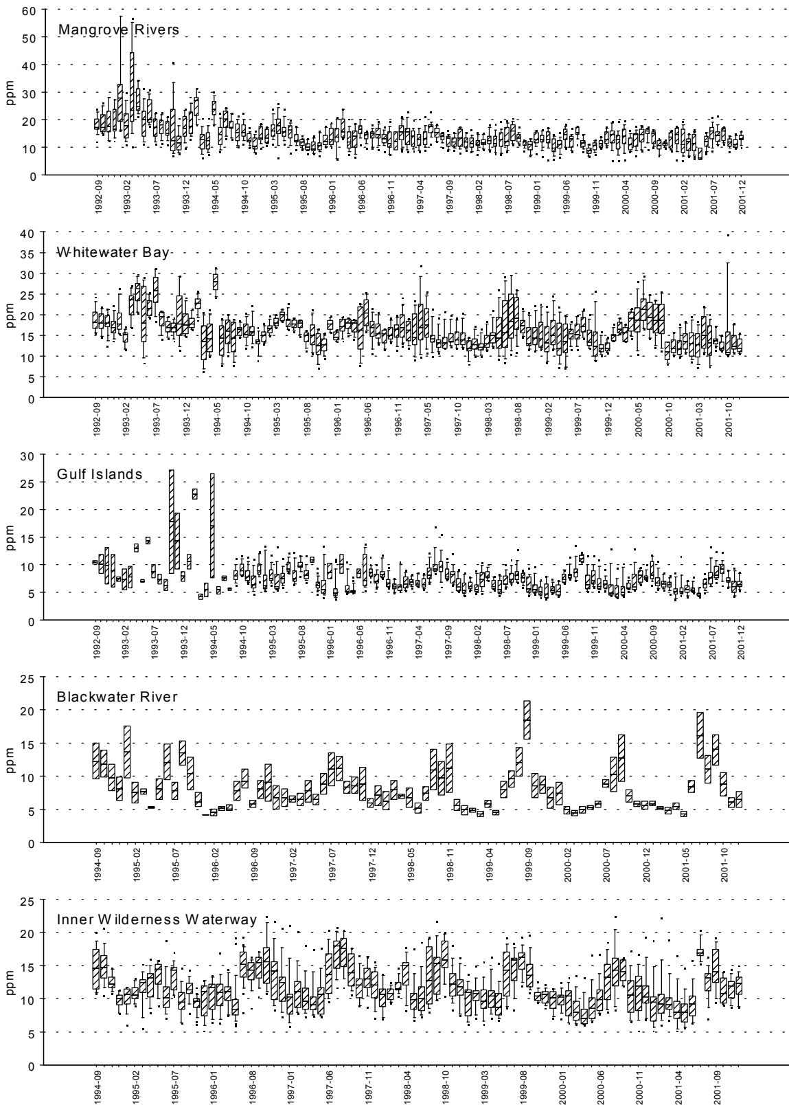
Figure 3.6. Monthly median and range of total organic carbon in the five WWB-TTI zones.
