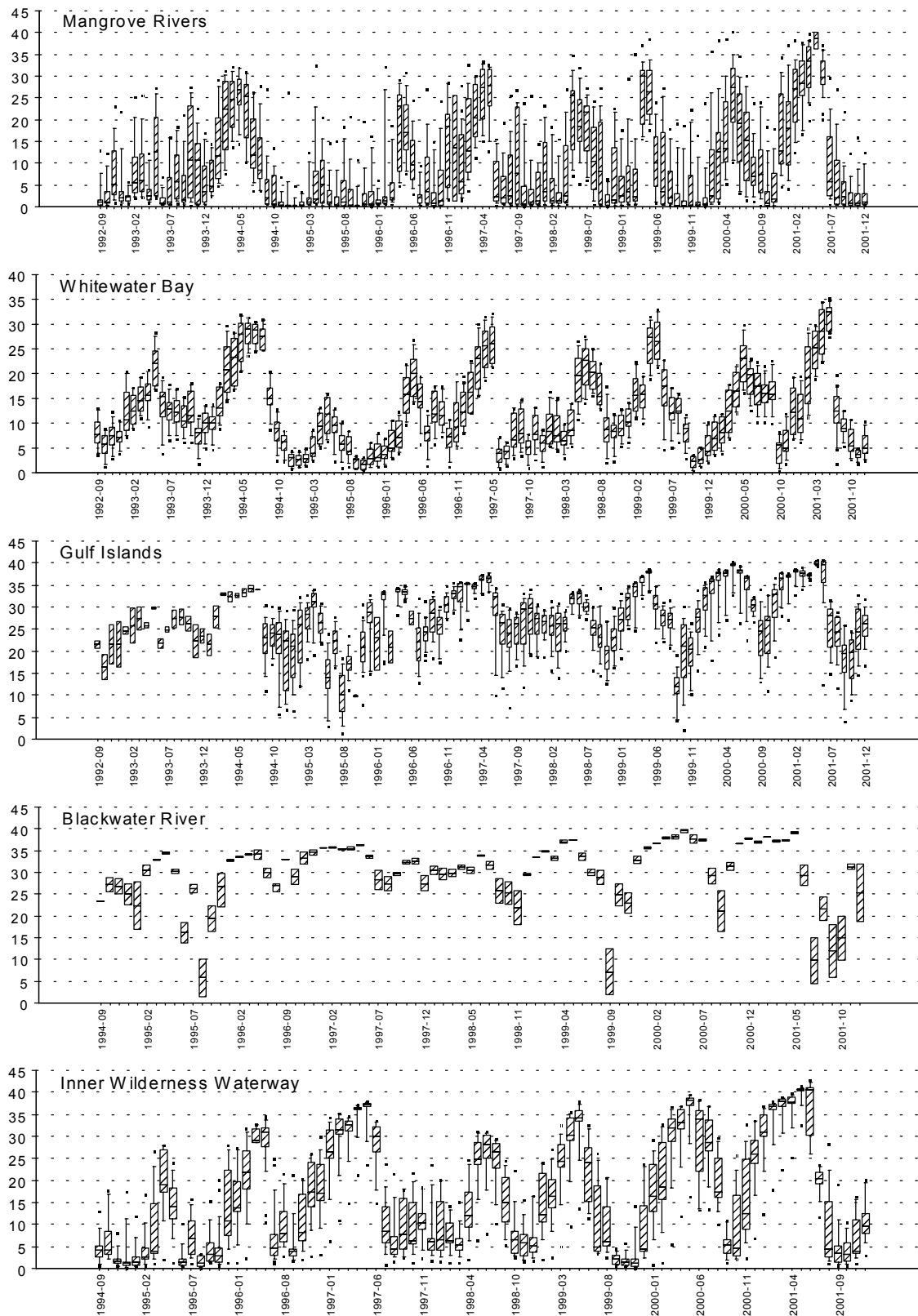
Figure 3.2. Monthly median and range of salinity in the five WTB-TTI zones.
