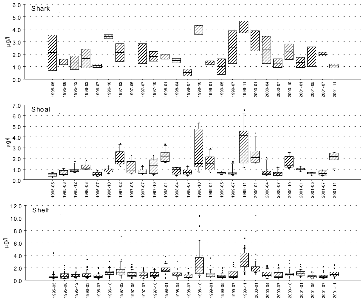
Figure 5.3. Quarterly median and range of chlorophyll a in the three SW Shelf zones.
