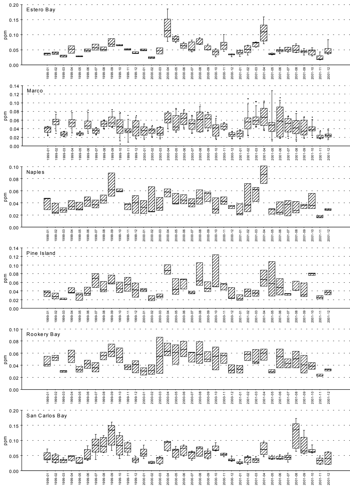
Figure 6.4. Monthly median and range of total phosphorus in the Cape Romano-PIS area.
