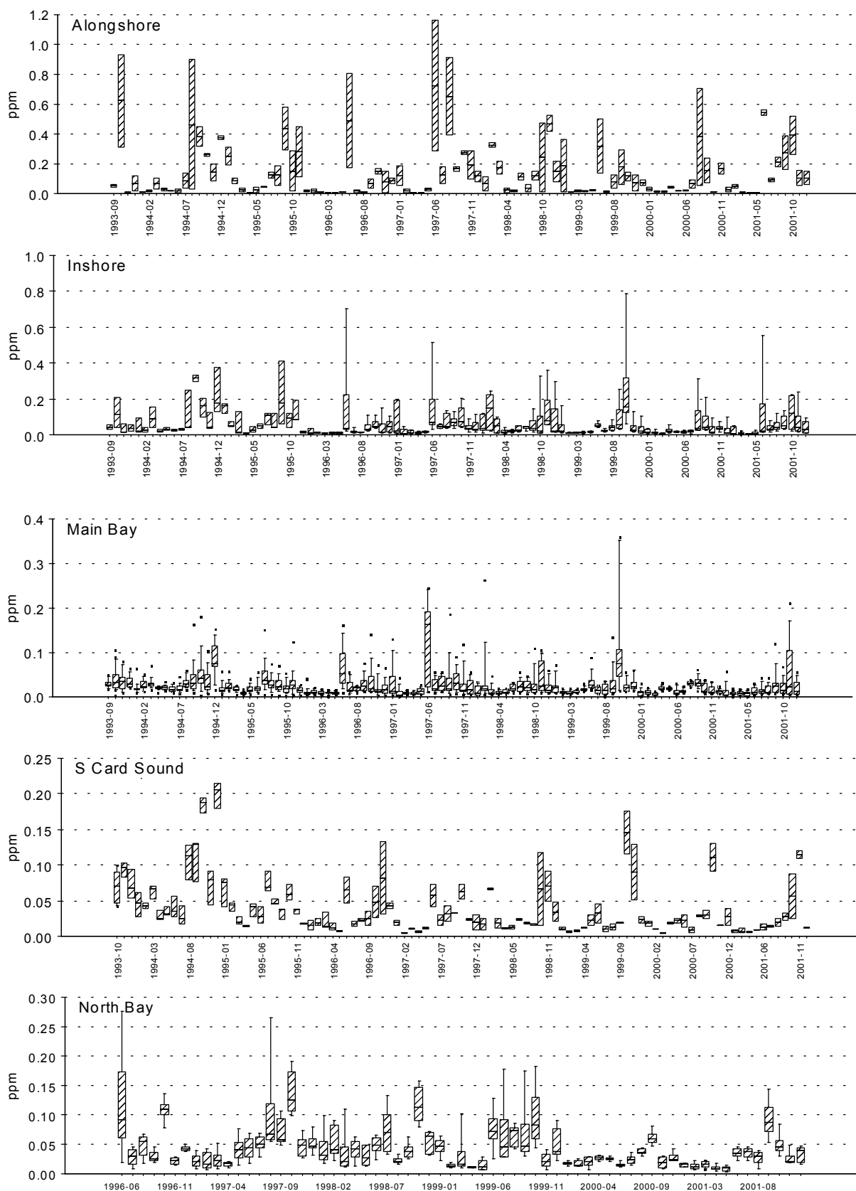
Figure 4.5. Monthly median and range of dissolved inorganic N in the Biscayne Bay zones.
