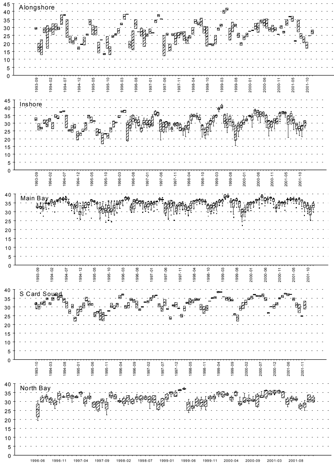
Figure 4.2. Monthly median and range of salinity in the five Biscayne Bay zones.
