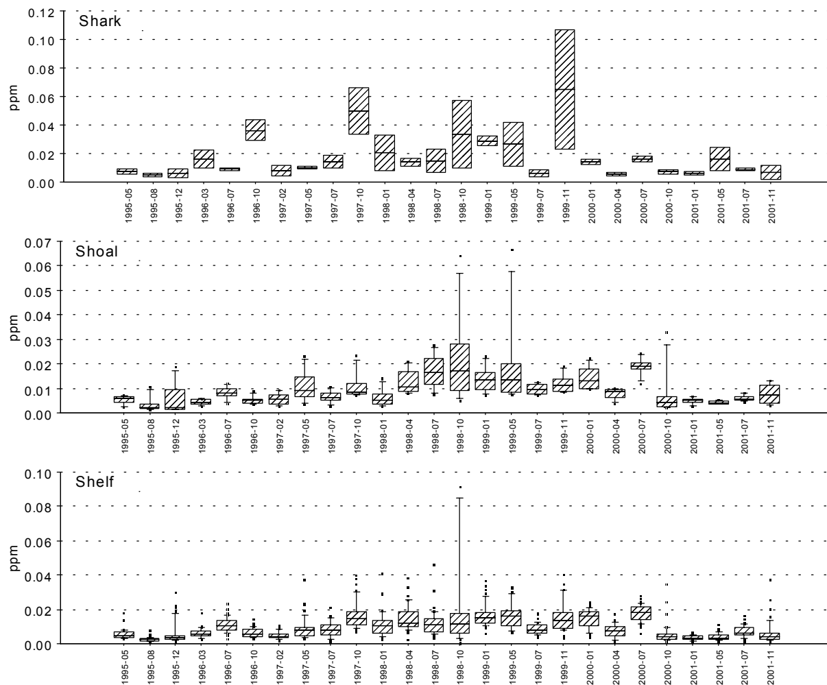
Figure 5.5. Quarterly median and range of dissolved inorganic N in the three SW Shelf zones.
