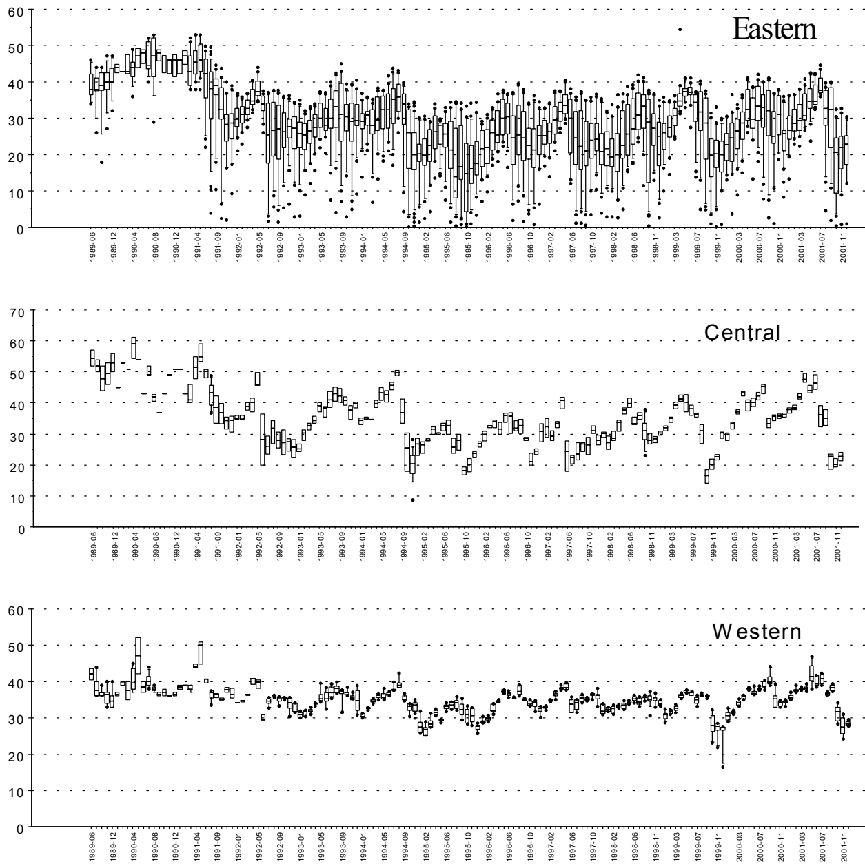
Figure 3. Monthly median and range of salinity in the three Florida Bay zones.
