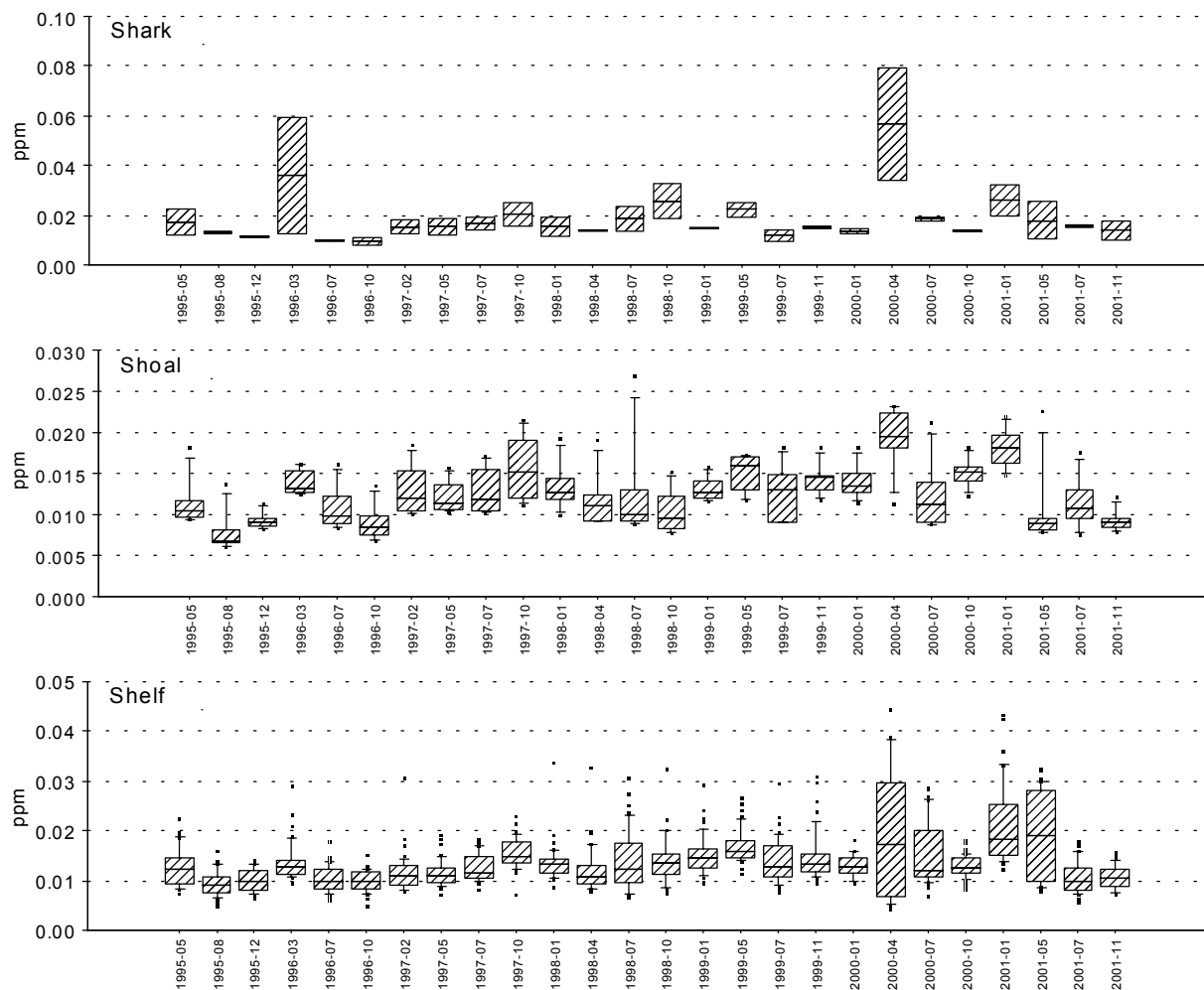
Figure 5.4. Quarterly median and range of total phosphorus in the three SW Shelf zones.
