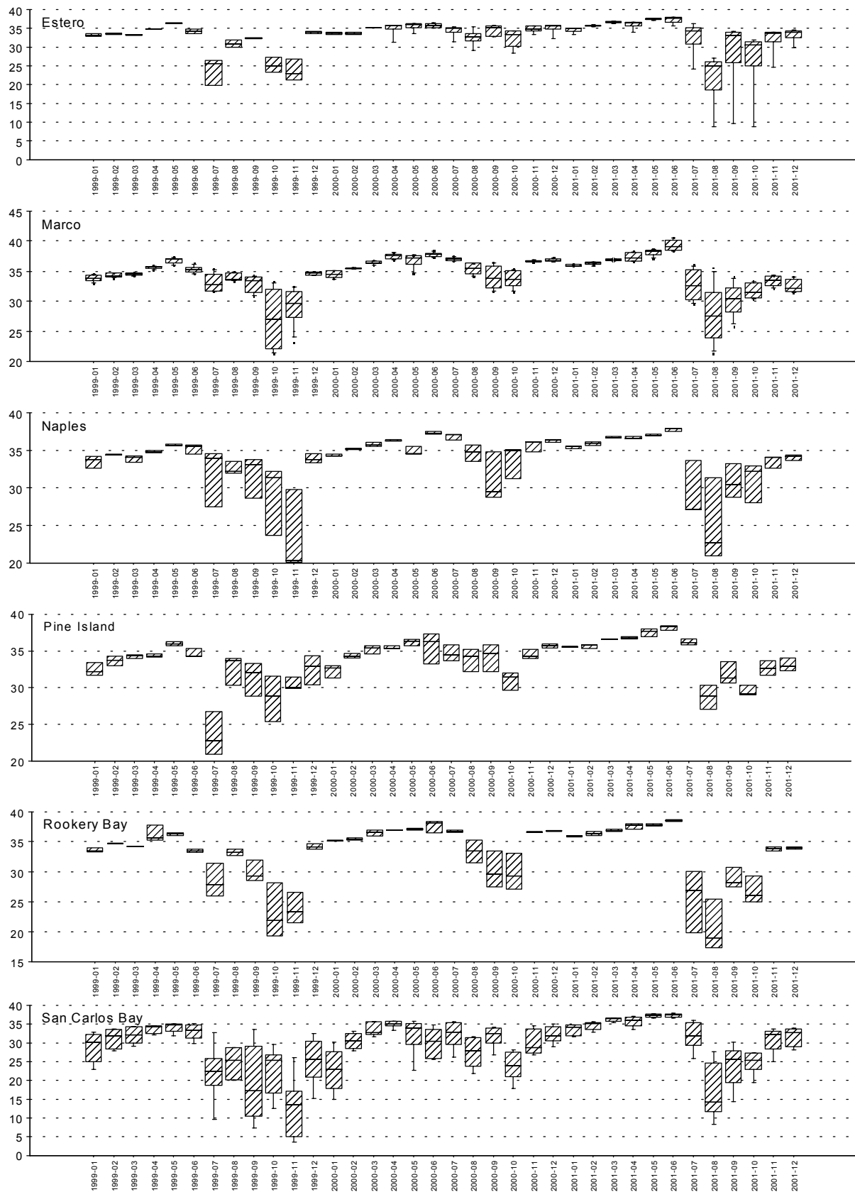
Figure 6.2. Monthly median and range of salinity in the Cape Romano-PIS area.
