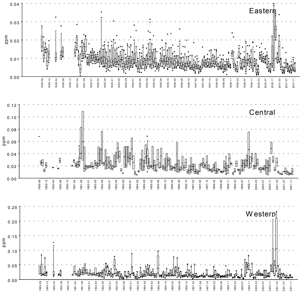
Figure 5. Monthly median and range of TP in the three Florida Bay zones.
