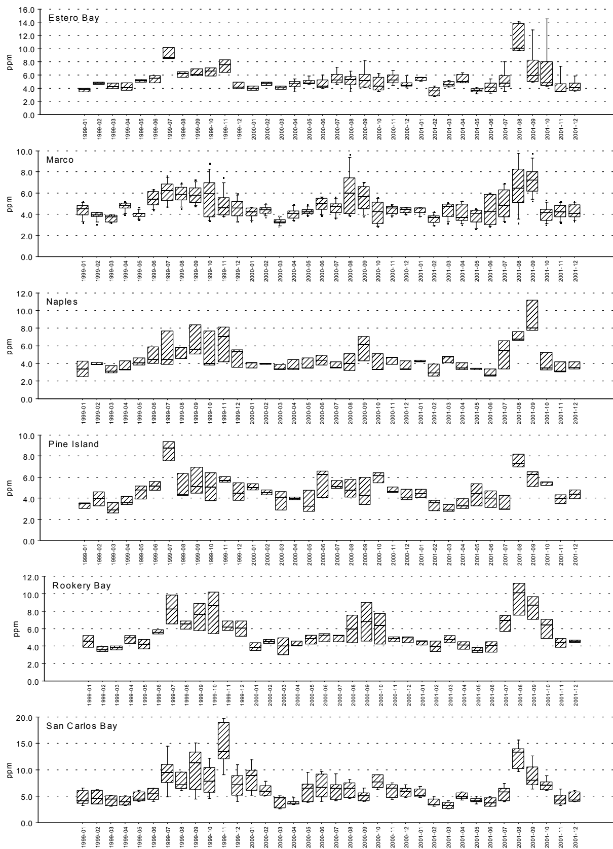
Figure 6.6. Monthly median and range of total organic carbon in the Cape Romano-PIS area.
