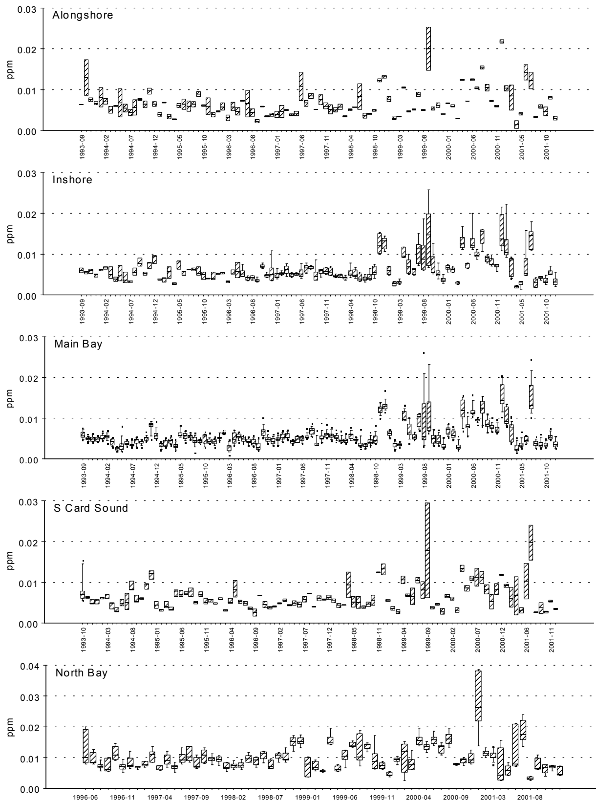
Figure 4.4. Monthly median and range of total phosphorus in the five Biscayne Bay zones.
