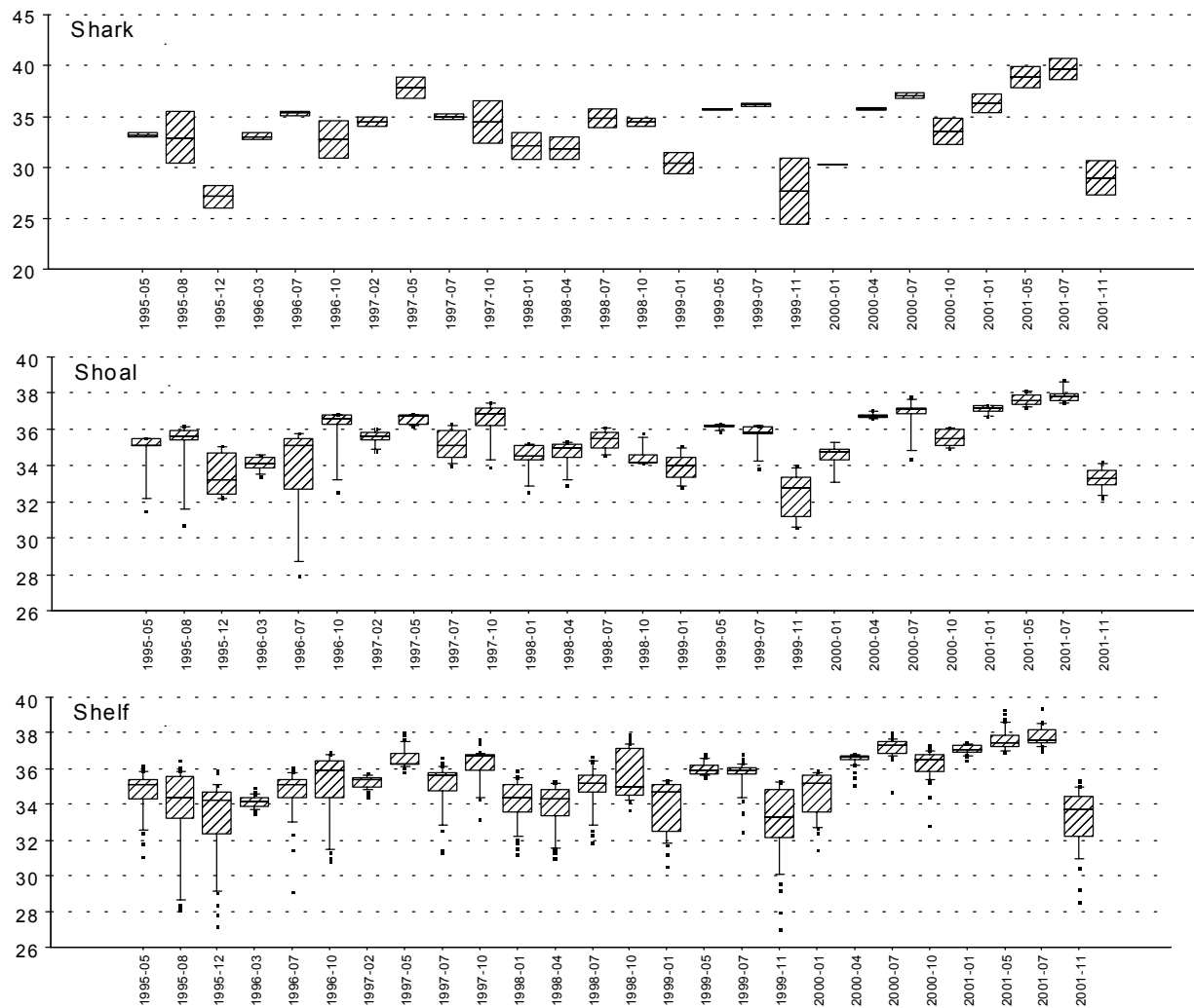
Figure 5.2. Quarterly median and range of salinity in the three SW Shelf zones.
