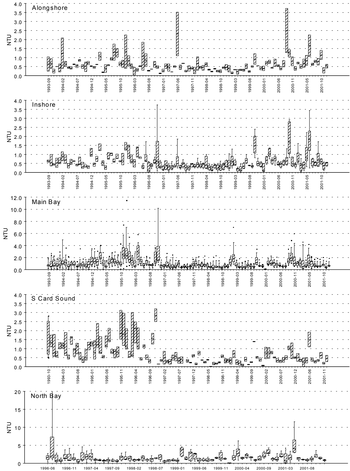
Figure 4.6. Monthly median and range of turbidity in the five Biscayne Bay zones.
