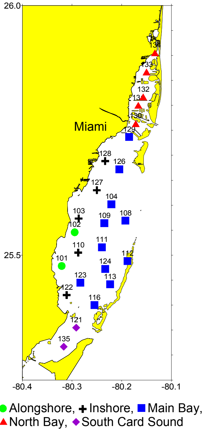
Figure 4.1. Zones of similar water quality in Biscayne Bay.
