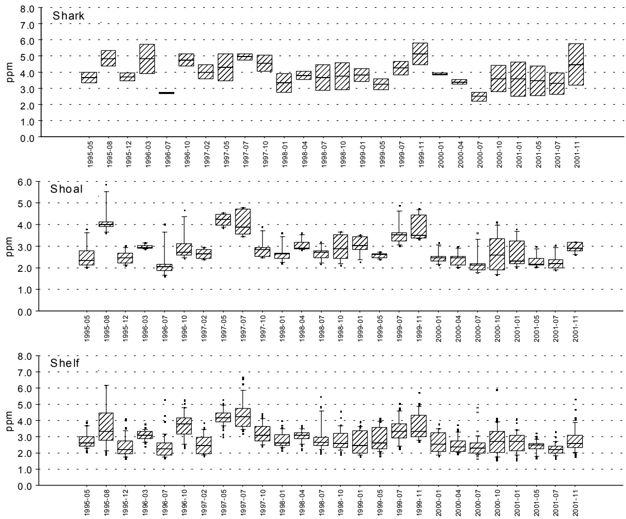
Figure 5.6. Quarterly median and range of total organic carbon in the three SW Shelf zones.
