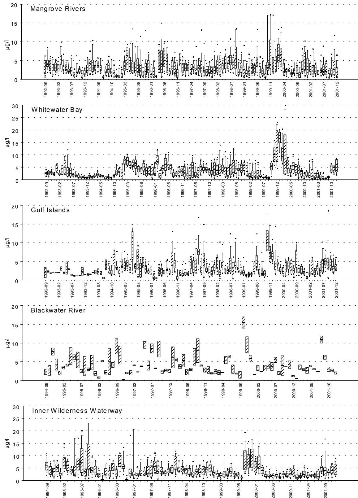
Figure 3.3. Monthly median and range of chlorophyll a in the five WWB-TTI zones.
