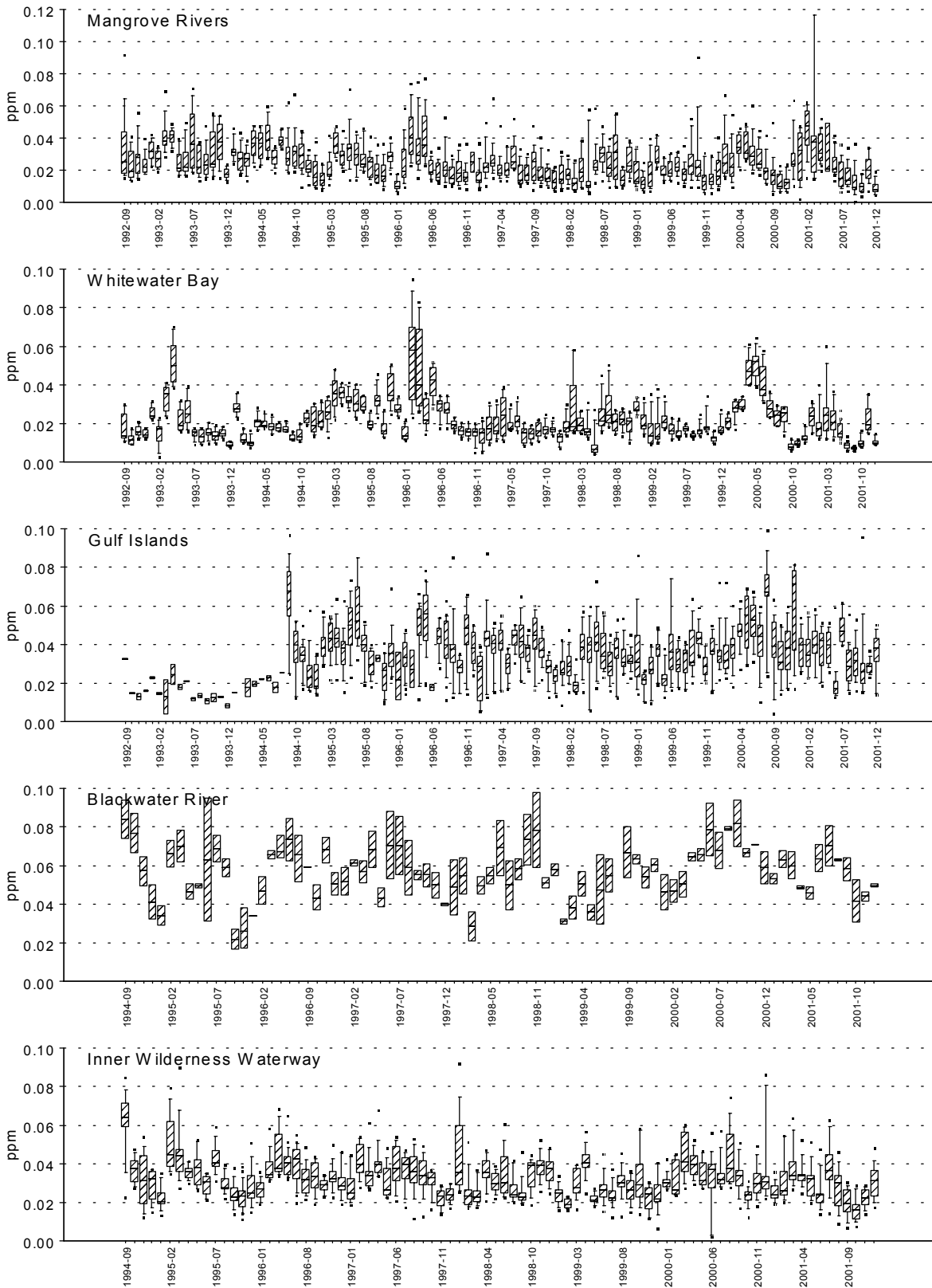
Figure 3.4. Monthly median and range of total phosphorus in the five WTB-TTI zones.
