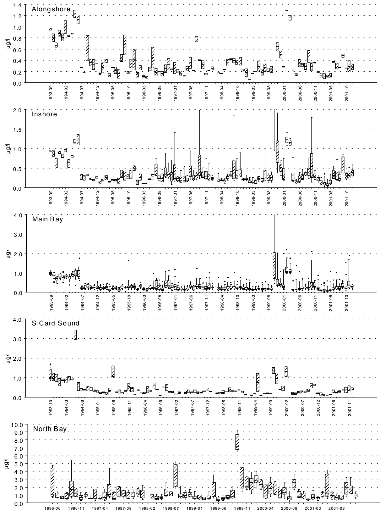
Figure 4.3. Monthly median and range of chlorophyll a in the five Biscayne Bay zones.
