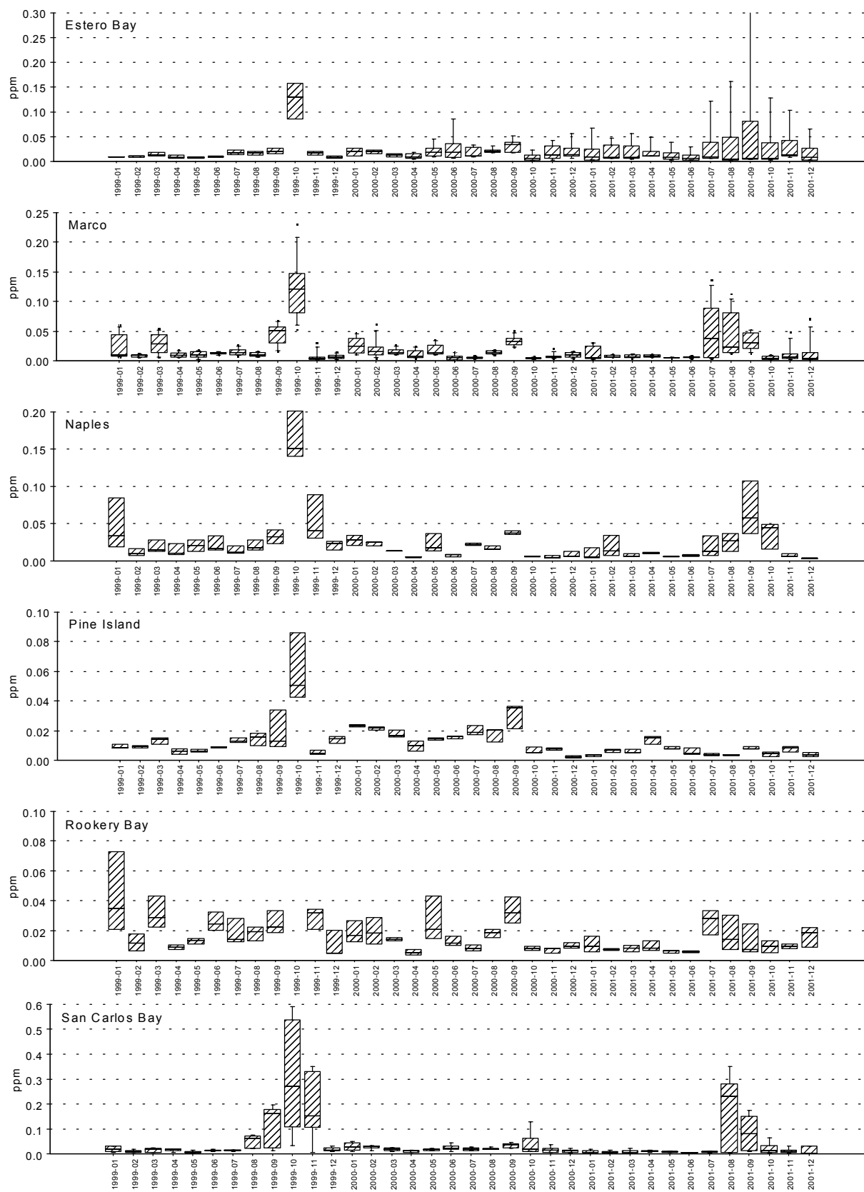
Figure 6.5. Monthly median and range of DIN in the Cape Romano-PIS area.
