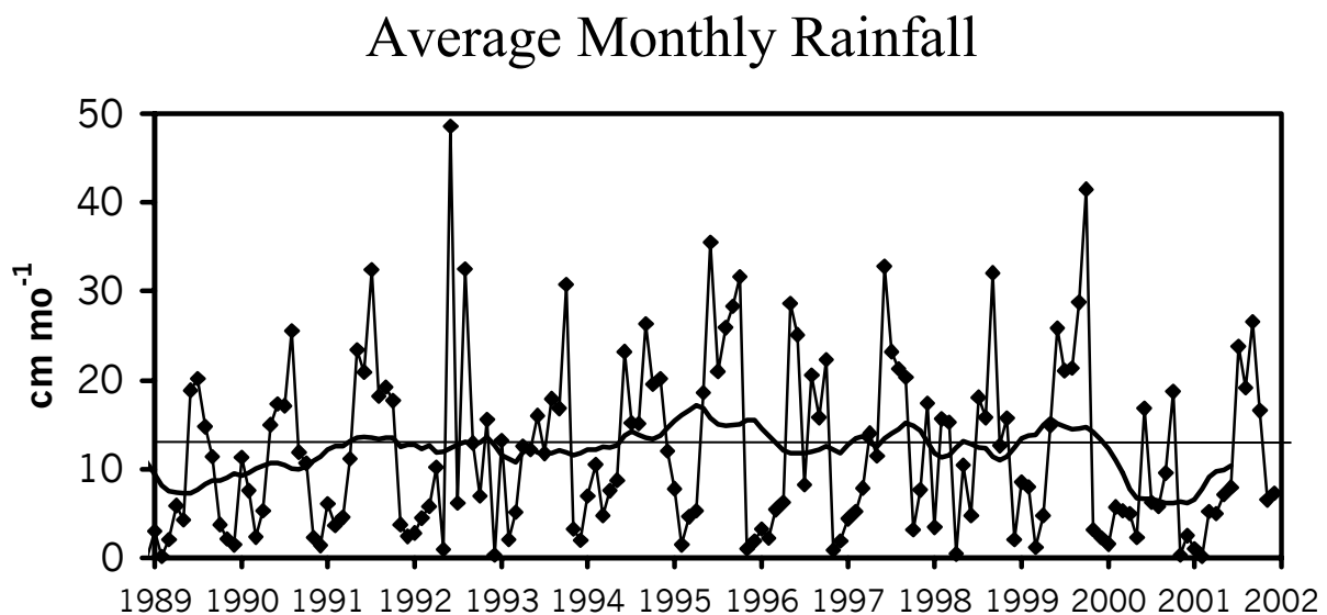
Figure 2. Monthly average rainfall in the Florida Bay area.
