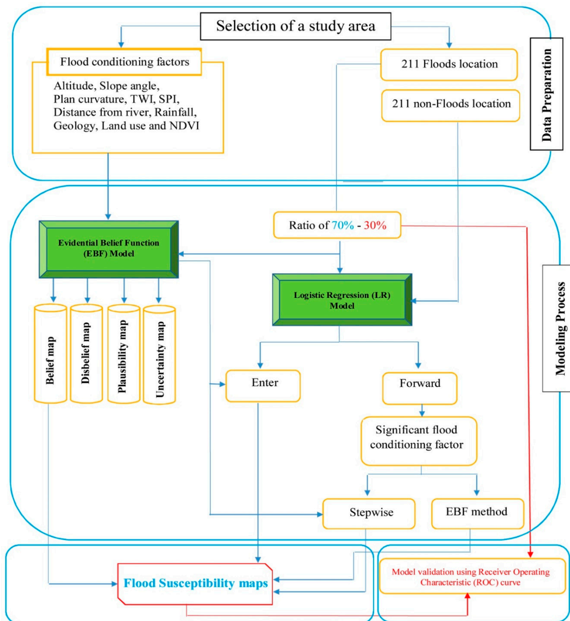
Figure 4. Flow chart of the adopted research methodology used to create flood susceptibility maps of the Haraz Catchment.
