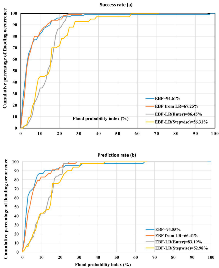
Figure 7. The success and prediction-rate curves for flooding map; (a) success rate and (b) prediction rate.
