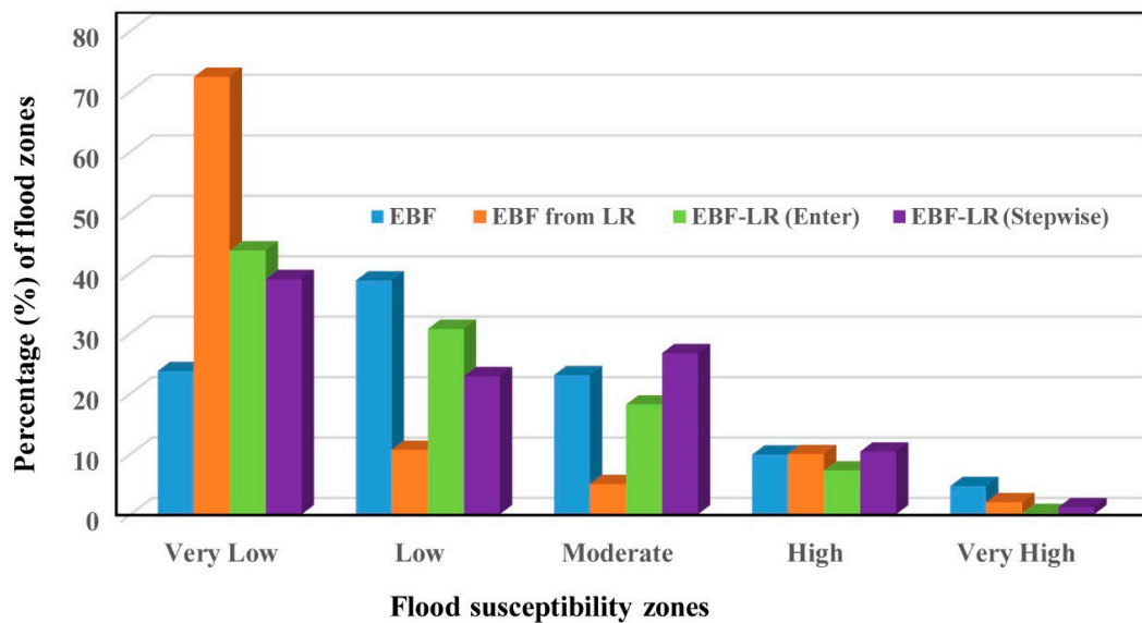
Figure 8. A histogram showing the percentage of flood zones that fall into the various classes from the four models.
