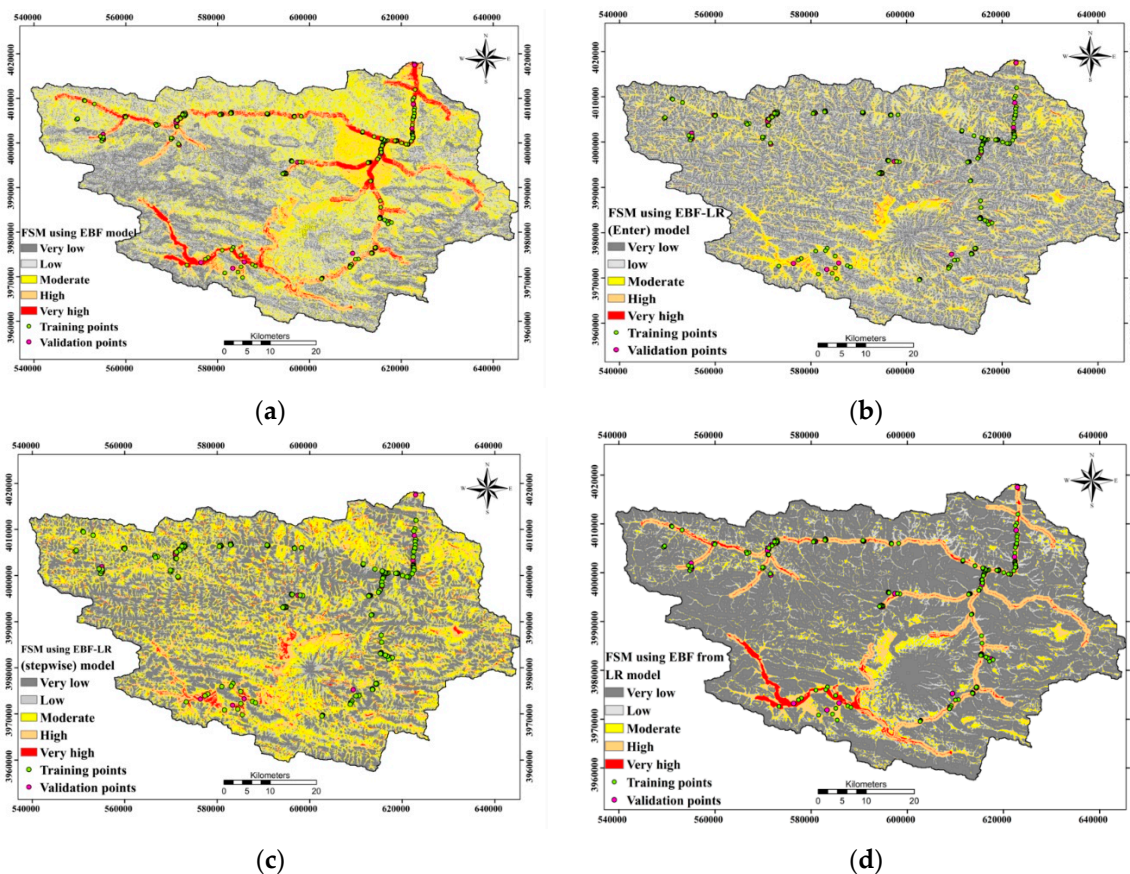
Figure 6. Flood Susceptibility Index using (a) EBF, (b) EBF-LR (Enter), (c) EBF-LR (Stepwise), (d) EBF from LR.
