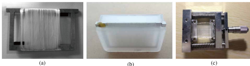
Fig. 3 Image from Ref. 107. (a) Cylinder model, (b) sphere-cylinder model, and (c) sphere-cylinder birefringence model.
