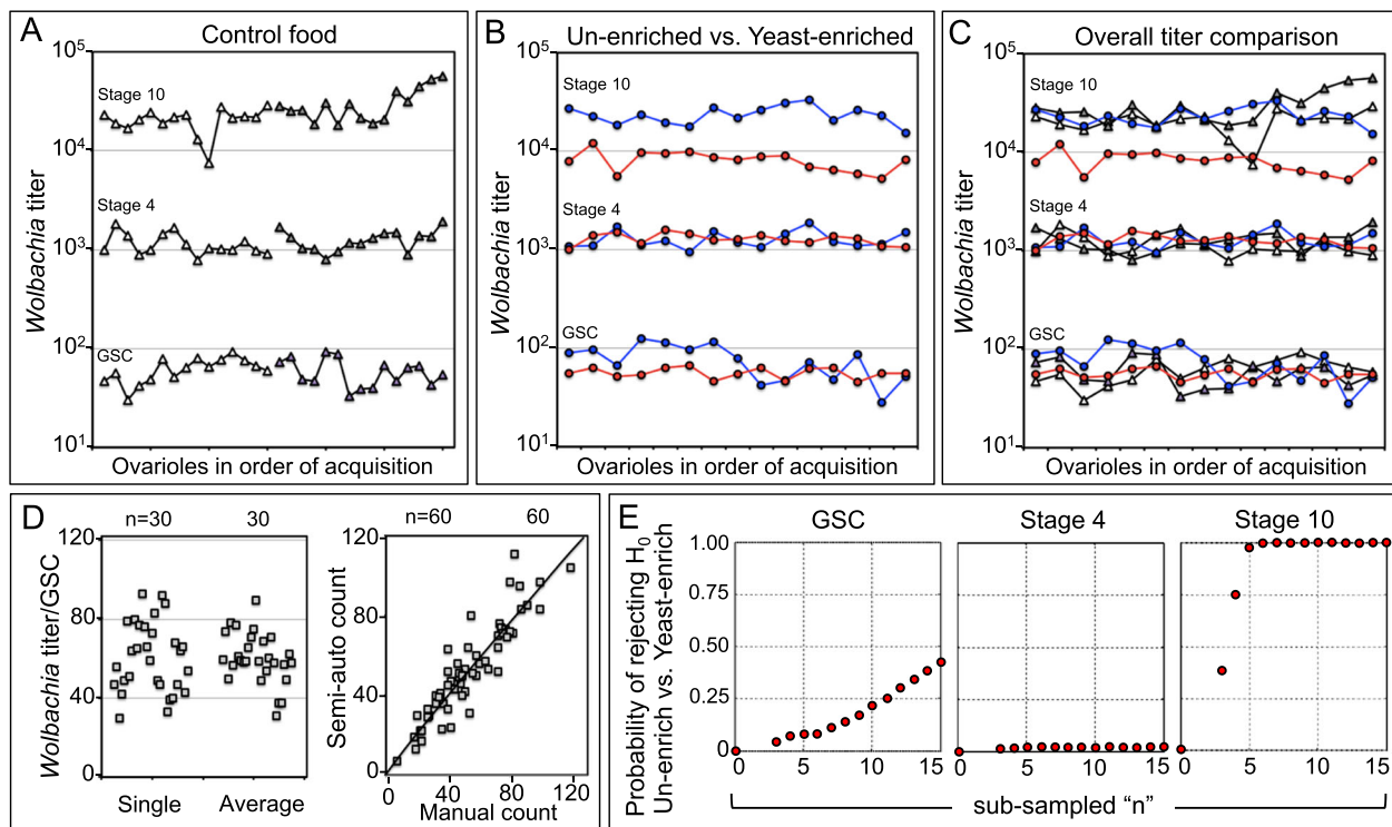
Fig. 4 Analysis of Wolbachia titer across oogenesis. GSC: Germline stem cell. a Titer data, displayed by stage and order of ovariole acquisition. White: First 15 ovarioles imaged. Grey: Last 15 ovarioles imaged. b Germline titer data in response to nutritional conditions. Blue: Un-enriched control. Red: Yeast-enriched treatment. c Overlay of all 3-dimensional titer data, in groups of 15 ovarioles. d Left: Comparison of control titer data for single GSCs versus median GSC titers scored in GSC clusters. Right: Comparison of data acquired by semi-automated versus manual assessment methods. Black line indicates regression analysis. e Comparing randomly sub-sampled data from un-enriched control and yeast-enriched treatment conditions. 10,000 iterations determined the frequency of significance, with alpha set at 0.01 ( n = 3-15 ovarioles). Tests used: Independent T-tests: GSCs and stage 10. Mann-Whitney U: stage 4
