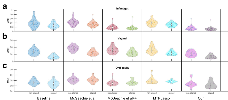
Fig. 4 Comparison of average predictive accuracy between methods on the filtered data sets. Figure shows violin plots of the MAE distributions of our proposed DBN models against a baseline method and previously published approaches for a sampling rate that most closely resembles the originally measured time points. Additionally, each method is run on the non-aligned and aligned data sets. a Performance results for infant gut microbiome data for sampling rate of 3 days. b Performance results for vaginal microbiome data for sampling rate of 3 days. c Performance results for oral cavity microbiome data for sampling rate of 7 days
