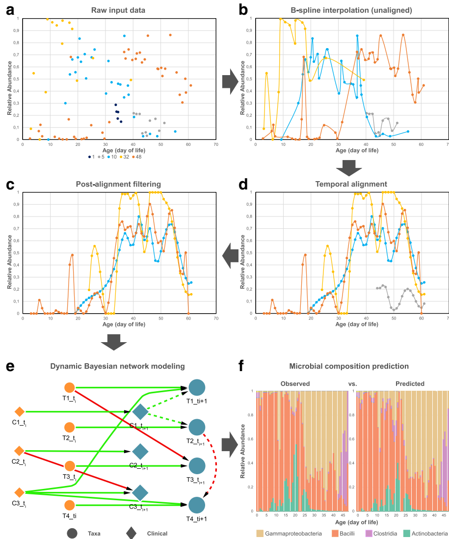
Fig. 1 Schematic diagram illustrating the whole computational pipeline proposed in this work. Figure shows microbial taxa Gammaproteobacteria at each step in the pipeline from a set of five representative individual samples (subjects 1, 5, 10, 32, and 48) of the gut data set. a Input is raw relative abundance values for each sample measured at (potentially) non-uniform intervals even within the same subject. b Cubic B-spline curve for each individual sample. Sample corresponding to subject 1 (dark blue) contains less than pre-defined threshold for measured time points, thus, removed from further analysis. The remaining smoothed curves enable principled estimation of unobserved time points and interpolation at uniform intervals. c Temporal alignment of each individual sample against a selected reference sample (subject 48 shown in orange). d Post-alignment filtering of samples with alignment error higher than a pre-defined threshold. Sample corresponding to subject 5 (grey) discarded. e Learning a dynamic Bayesian network (DBN) structure and parameters. Let nodes ( T_1, T_2, T_3, T_4 ) represent microbial taxa and ( C_1, C_2, C_3 ) represent clinical factors shown as circles and diamonds, respectively. Figure shows two consecutive time slices t_i and t_{i+1} , where dotted lines connect nodes from the same time slice referred to as intra edges , and solid lines connect nodes between time slices referred to as inter edges . Biological relationships are inferred from edge parameters in the learned DBN which can be positive (green) or negative (red). f Original and predicted relative abundance across four gut taxa for subject 48 at sampling rate of 1 day. Performance is evaluated by average mean absolute error (MAE) between original and predicted abundance values (MAE = 0.011)
