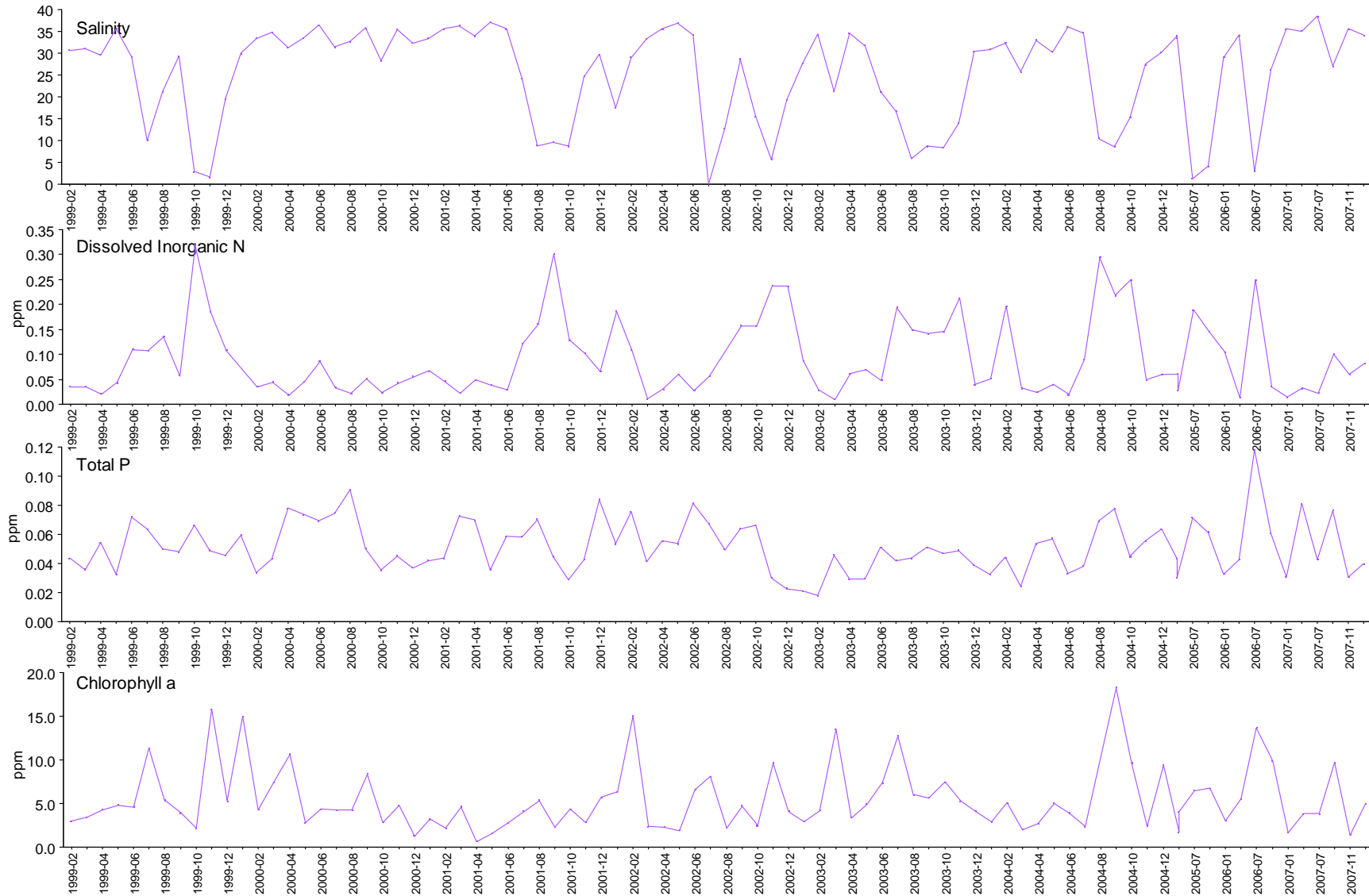
Figure 4.5.8. Single point times series of water quality in the Cocohatchee River by survey.
