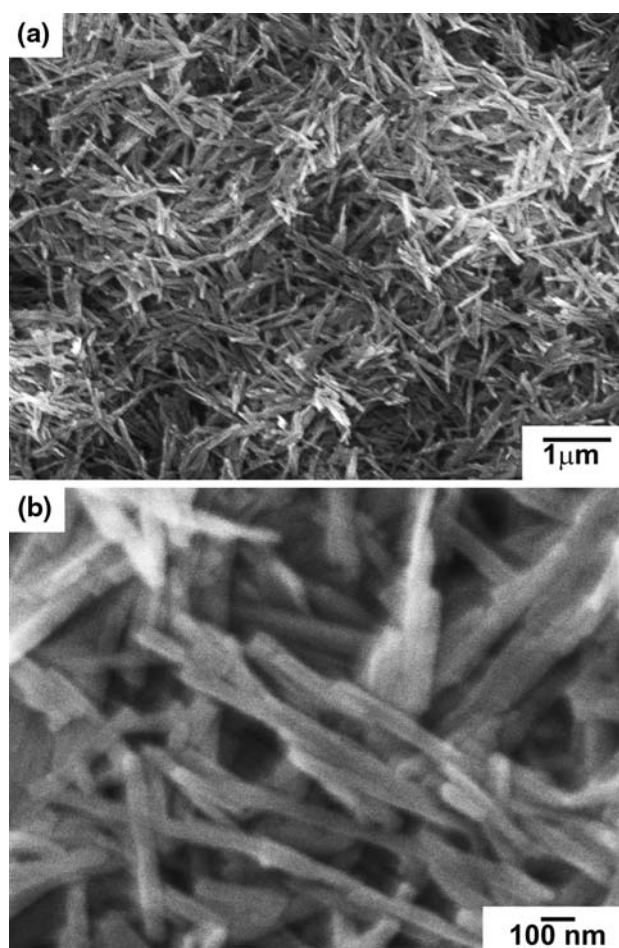
Fig. 2 a Low- and b high-magnification SEM images of magnesium borate hydroxide nanowhiskers fabricated without surfactant
