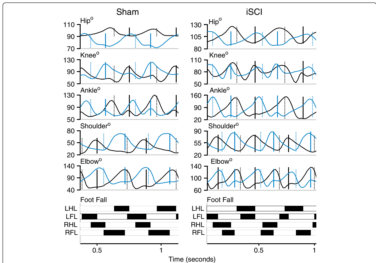
Figure 3 Example locomotor kinematics during treadmill walking. Joint angle kinematics and footfall measures during treadmill walking from one sham and one iSCI animal (T9 spinal level), 4 weeks post injury. The black traces are for the left limb and the blue traces are for the right limb. The solid vertical lines are touchdown and the dotted vertical lines are lift-off. For footfall, the black sections represent swing and the white sections stance. LHL, left hindlimb; LFL, left forelimb; RHL, right hindlimb; and RFL, right forelimb. Note the decrease in the magnitude of the second local maxima of the ankle trajectory in the contusion animal as well as the inconsistent step pattern.
