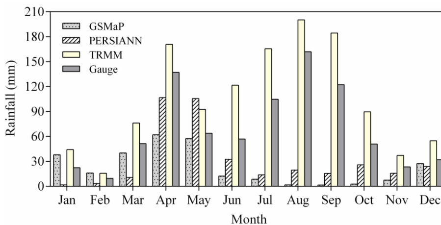
Figure 6. Monthly average rainfall (2003–2006) from GSMaP, PERSIANN, and TRMM averaged over selected grid cells with rain gauge data.
