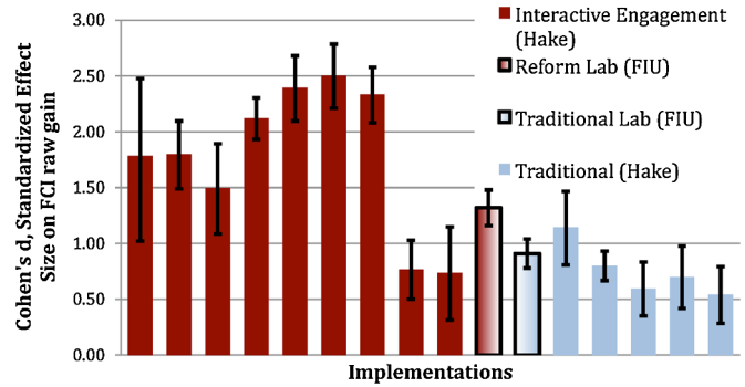
FIG. 1 (color online). A comparison of Cohen's d standardized effect sizes on raw gain on the Force Concept Inventory from various instructional strategies. The data include effect sizes of interactive-engagement courses reported by Hake [1] in red and effect sizes of traditional courses reported by Hake in blue; the categories were determined by Hake and only university data are included. We report FIU results for transformed labs (shaded red) and traditional labs (shaded blue). Error bars represent 95% confidence intervals on the effect size.
