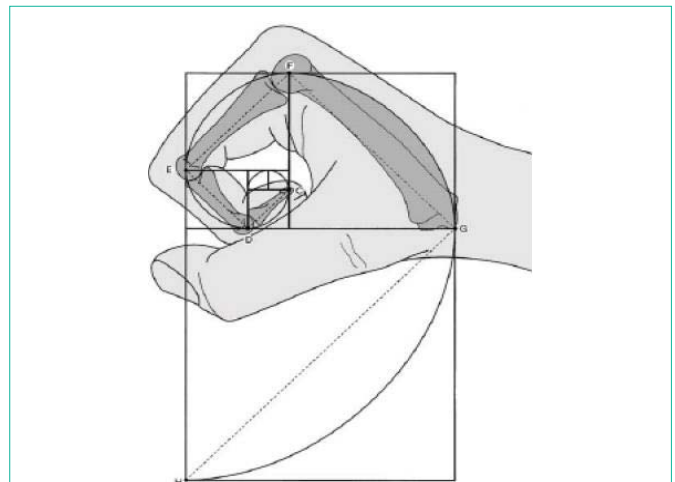
Figure 4: The human hand superimposed on the Golden Rectangle, with approximations to the Golden Spiral [4].
